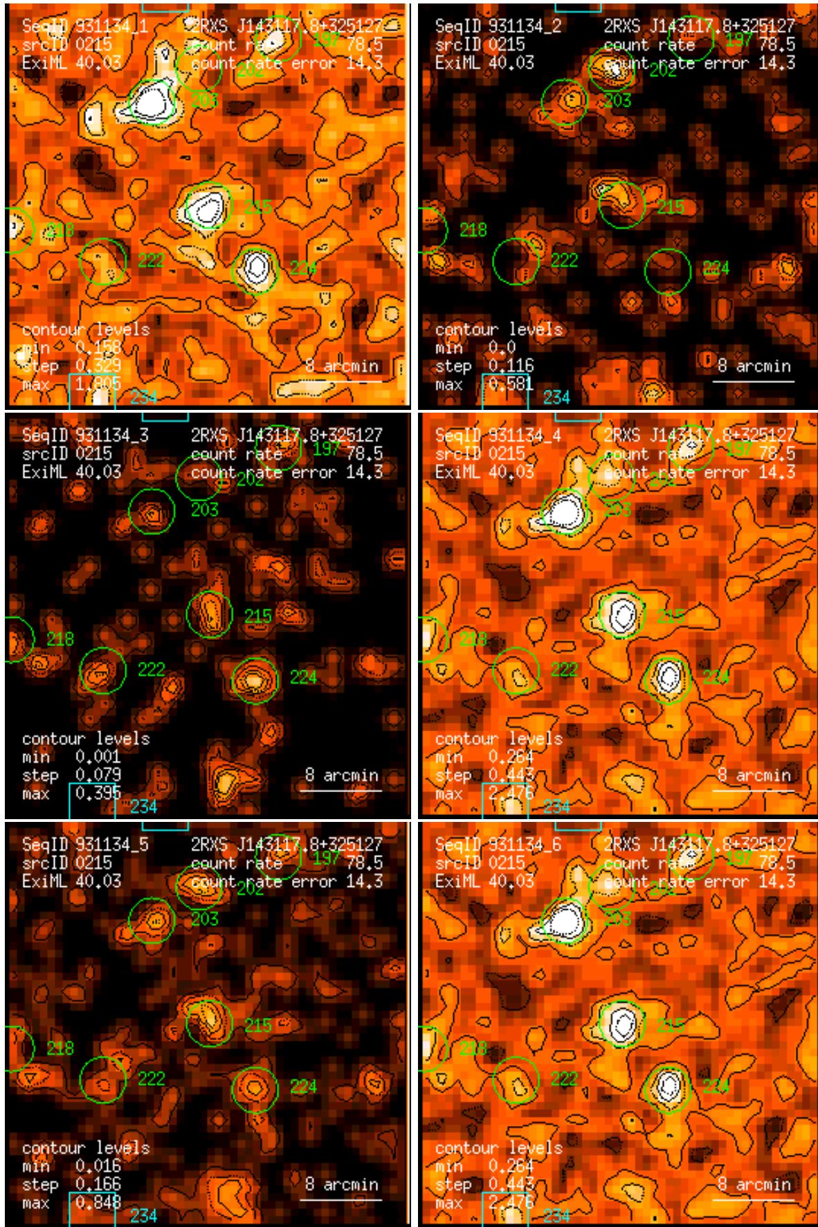
Figure 215: RASS 931134: detection 0215: band rate images, Gaussian filter: (1) PSPC channels 11 – 41, (2) 52 – 90, (3) 91 – 201, (4) 11 – 235, (5) 52 – 201, (6) 11 – 201. Broad band rates in counts/ks. Band rate contour levels in counts/ks/arcmin 2 .
