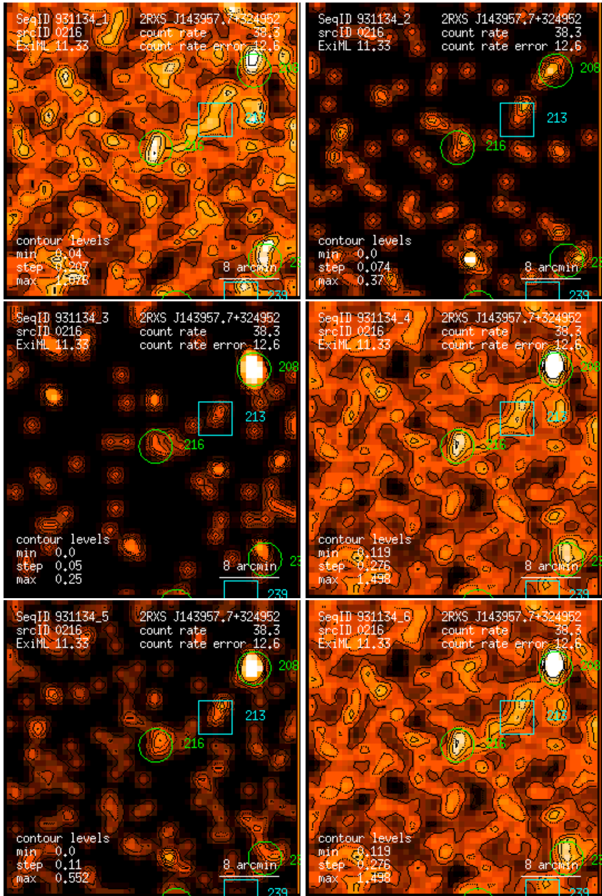
Figure 216: RASS 931134: detection 0216: band rate images, Gaussian filter: (1) PSPC channels 11 – 41, (2) 52 – 90, (3) 91 – 201, (4) 11 – 235, (5) 52 – 201, (6) 11 – 201. Broad band rates in counts/ks. Band rate contour levels in counts/ks/arcmin 2 .
