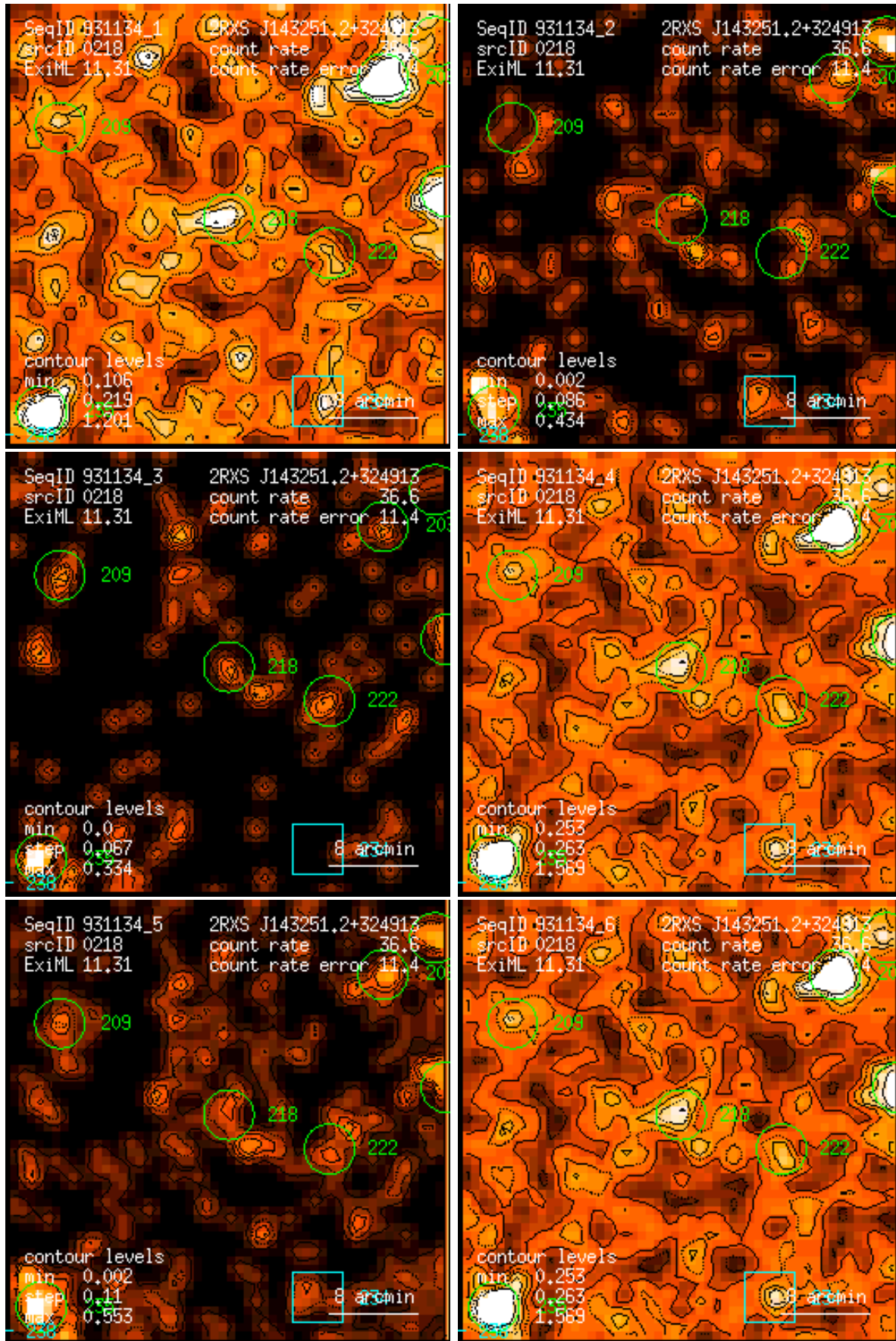
Figure 218: RASS 931134: detection 0218: band rate images, Gaussian filter: (1) PSPC channels 11 – 41, (2) 52 – 90, (3) 91 – 201, (4) 11 – 235, (5) 52 – 201, (6) 11 – 201. Broad band rates in counts/ks. Band rate contour levels in counts/ks/arcmin 2 .
