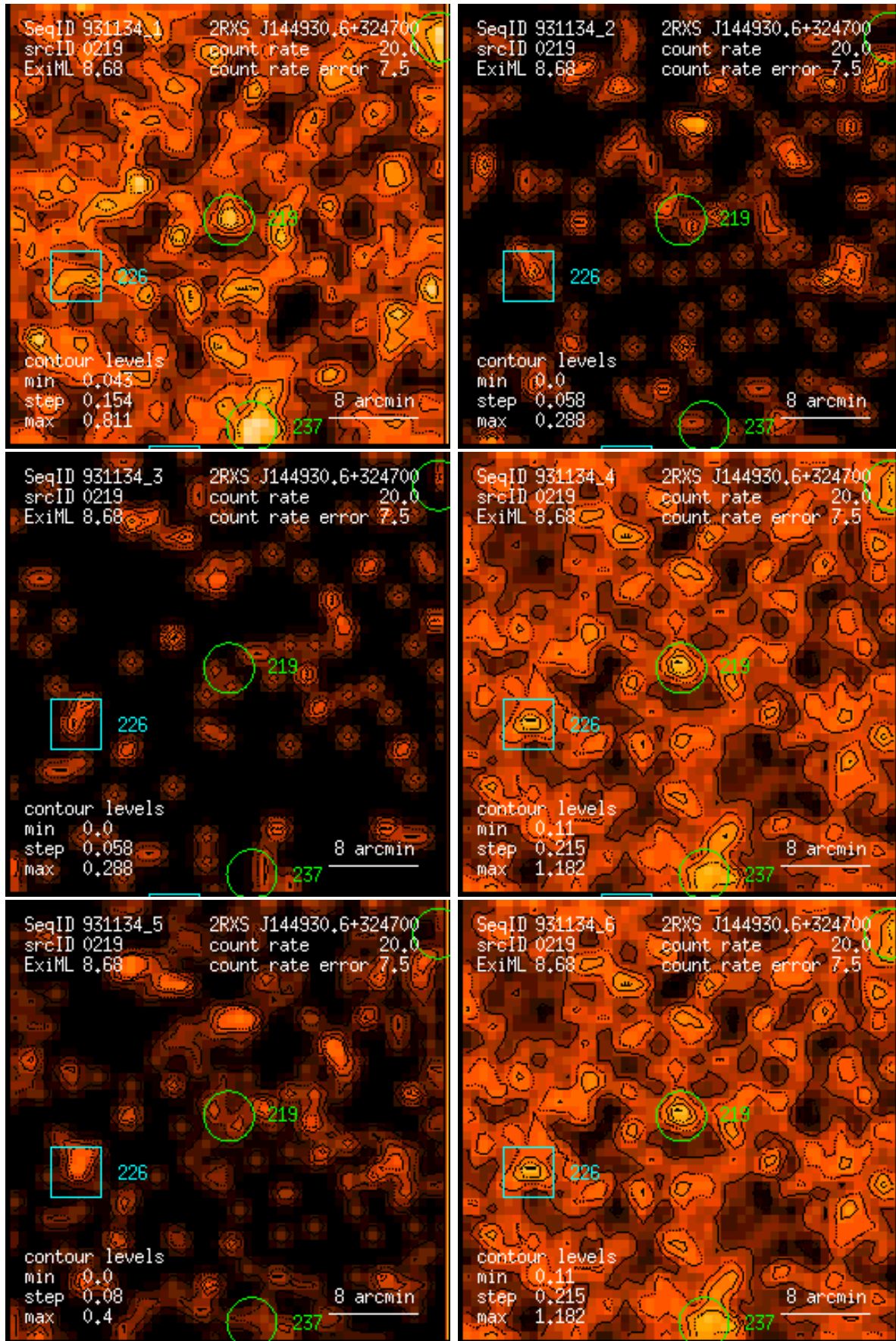
Figure 219: RASS 931134: detection 0219: band rate images, Gaussian filter: (1) PSPPC channels 11 – 41, (2) 52 – 90, (3) 91 – 201, (4) 11 – 235, (5) 52 – 201, (6) 11 – 201. Broad band rates in counts/ks. Band rate contour levels in counts/ks/arcmin 2 .
