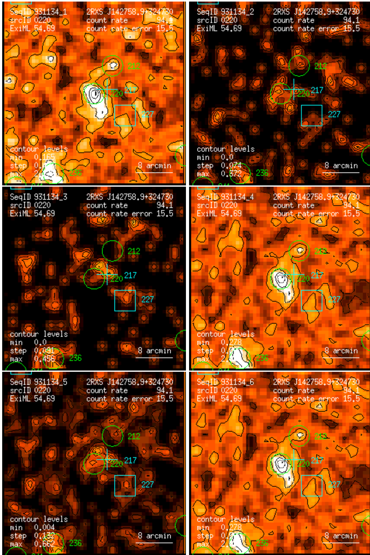
Figure 220: RASS 931134: detection 0220: band rate images, Gaussian filter: (1) PSPC channels 11 – 41, (2) 52 – 90, (3) 91 – 201, (4) 11 – 235, (5) 52 – 201, (6) 11 – 201. Broad band rates in counts/ks. Band rate contour levels in counts/ks/arcmin 2 .
