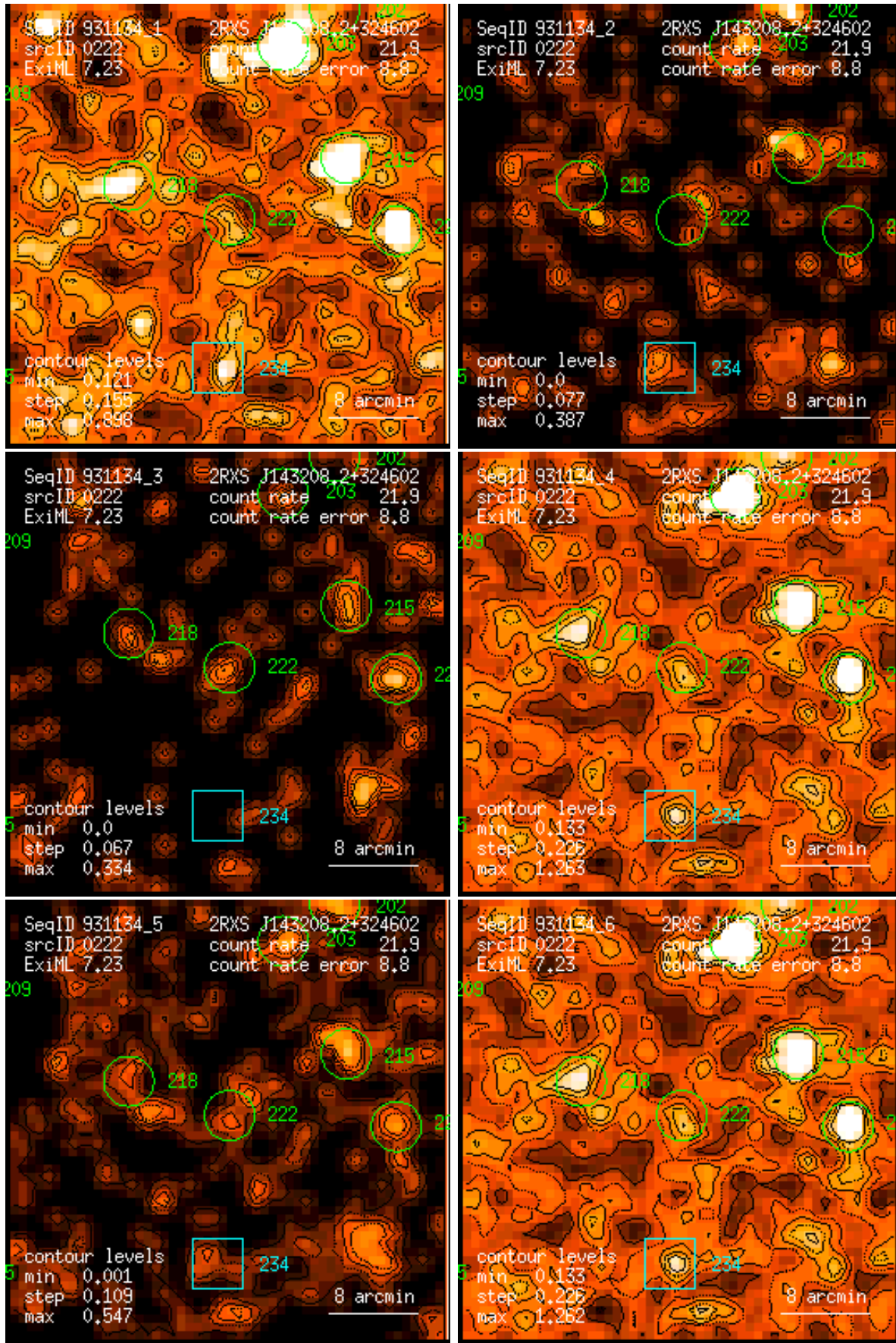
Figure 222: RASS 931134: detection 0222: band rate images, Gaussian filter: (1) PSPC channels 11 – 41, (2) 52 – 90, (3) 91 – 201, (4) 11 – 235, (5) 52 – 201, (6) 11 – 201. Broad band rates in counts/ks. Band rate contour levels in counts/ks/arcmin 2 .
