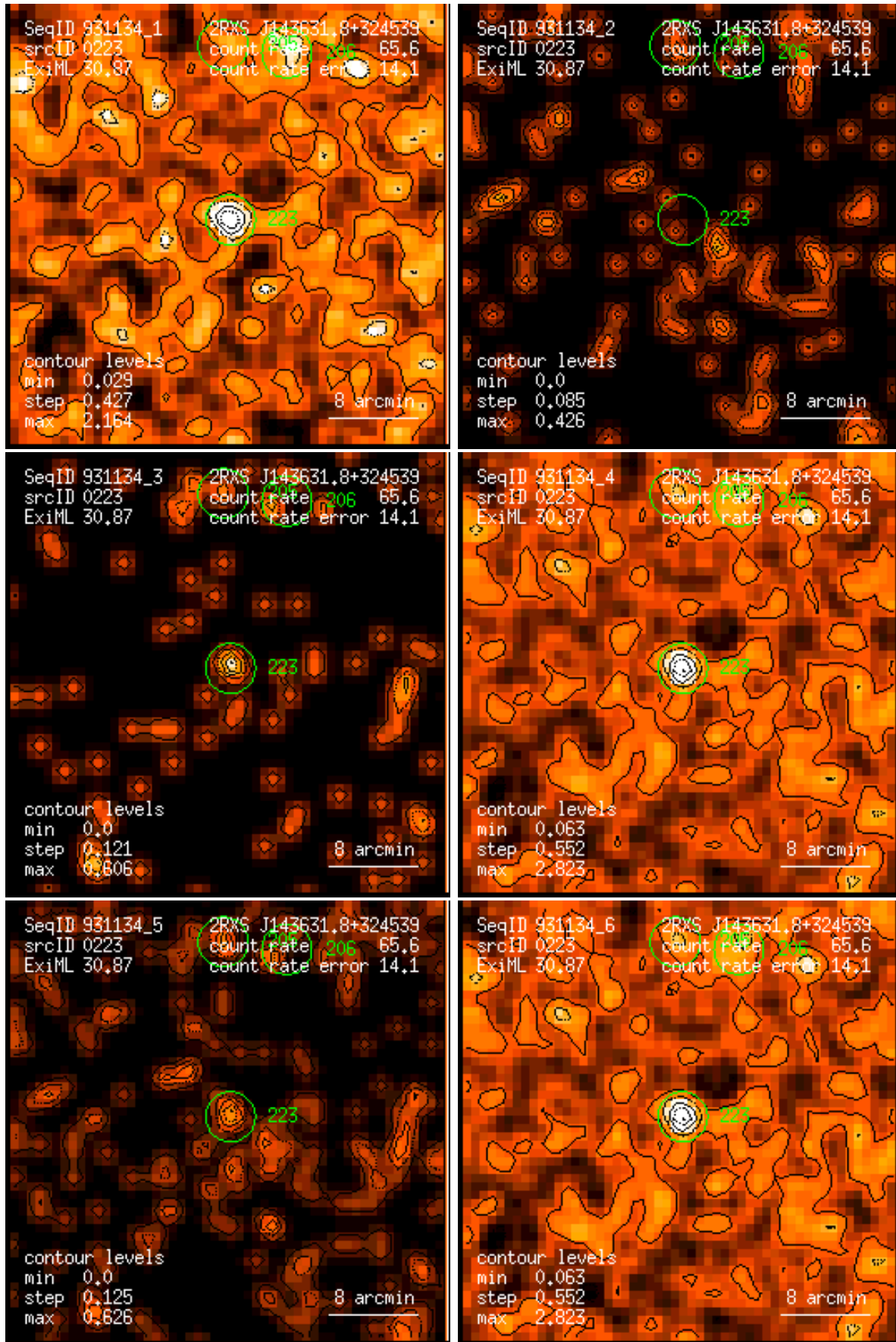
Figure 223: RASS 931134: detection 0223: band rate images, Gaussian filter: (1) PSPC channels 11 – 41, (2) 52 – 90, (3) 91 – 201, (4) 11 – 235, (5) 52 – 201, (6) 11 – 201. Broad band rates in counts/ks. Band rate contour levels in counts/ks/arcmin 2 .
