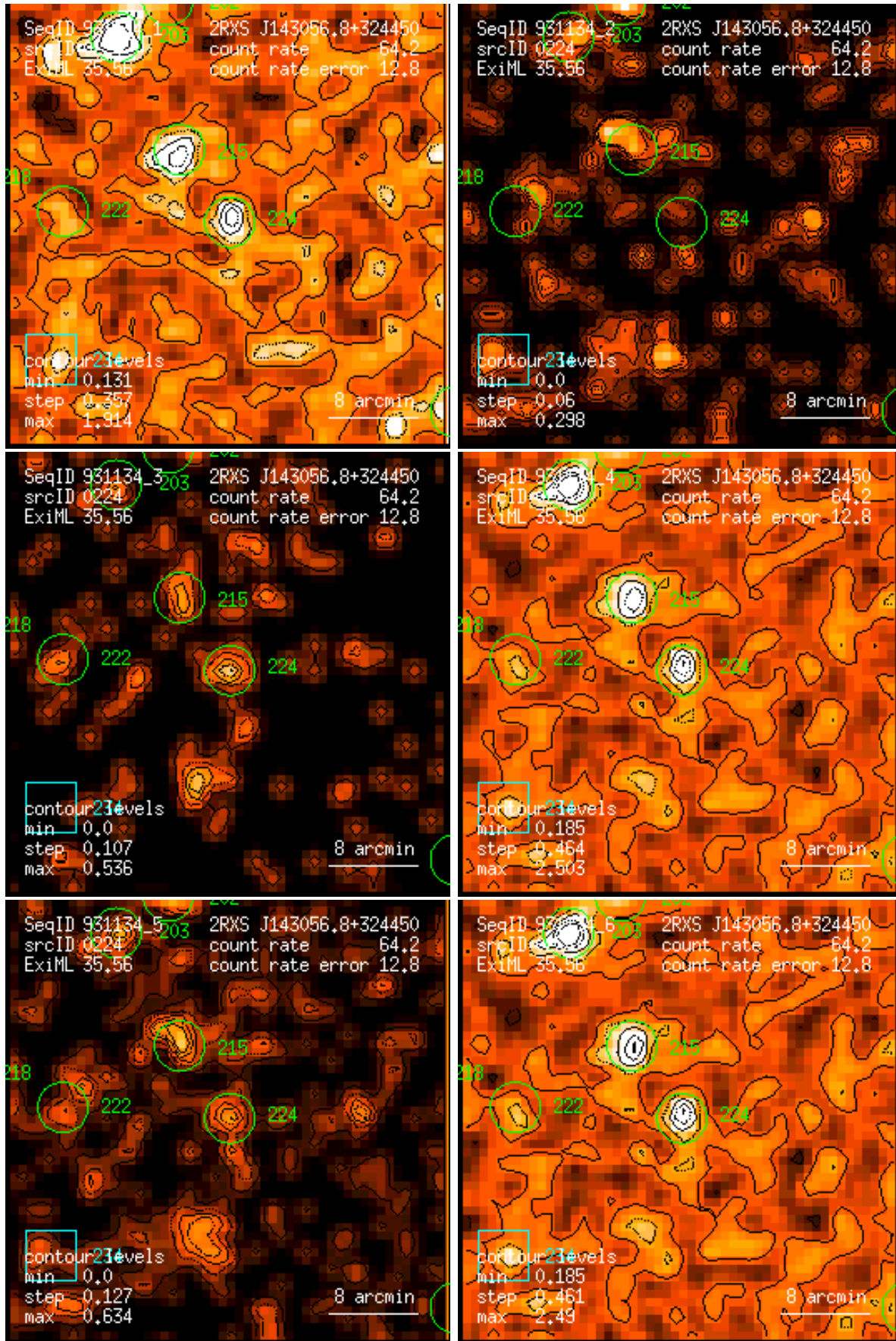
Figure 224: RASS 931134: detection 0224: band rate images, Gaussian filter: (1) PSPC channels 11 – 41, (2) 52 – 90, (3) 91 – 201, (4) 11 – 235, (5) 52 – 201, (6) 11 – 201. Broad band rates in counts/ks. Band rate contour levels in counts/ks/arcmin 2 .
