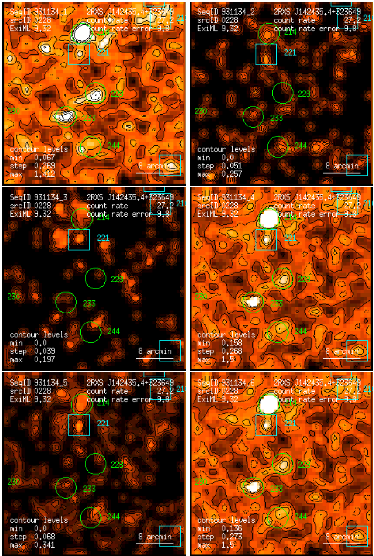
Figure 228: RASS 931134: detection 0228: band rate images, Gaussian filter: (1) PSPC channels 11 – 41, (2) 52 – 90, (3) 91 – 201, (4) 11 – 235, (5) 52 – 201, (6) 11 – 201. Broad band rates in counts/ks. Band rate contour levels in counts/ks/arcmin 2 .
