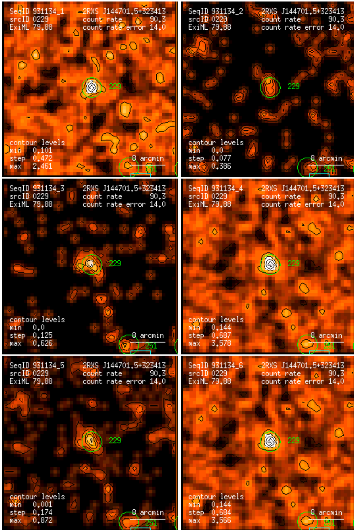
Figure 229: RASS 931134: detection 0229: band rate images, Gaussian filter: (1) PSPC channels 11 – 41, (2) 52 – 90, (3) 91 – 201, (4) 11 – 235, (5) 52 – 201, (6) 11 – 201. Broad band rates in counts/ks. Band rate contour levels in counts/ks/arcmin 2 .
