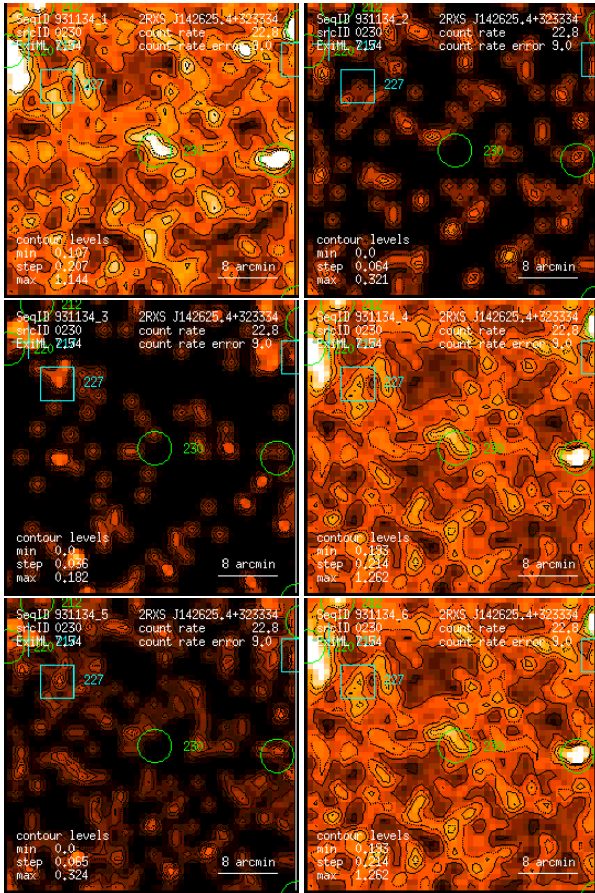
Figure 230: RASS 931134: detection 0230: band rate images, Gaussian filter: (1) PSPC channels 11 – 41, (2) 52 – 90, (3) 91 – 201, (4) 11 – 235, (5) 52 – 201, (6) 11 – 201. Broad band rates in counts/ks. Band rate contour levels in counts/ks/arcmin 2 .
