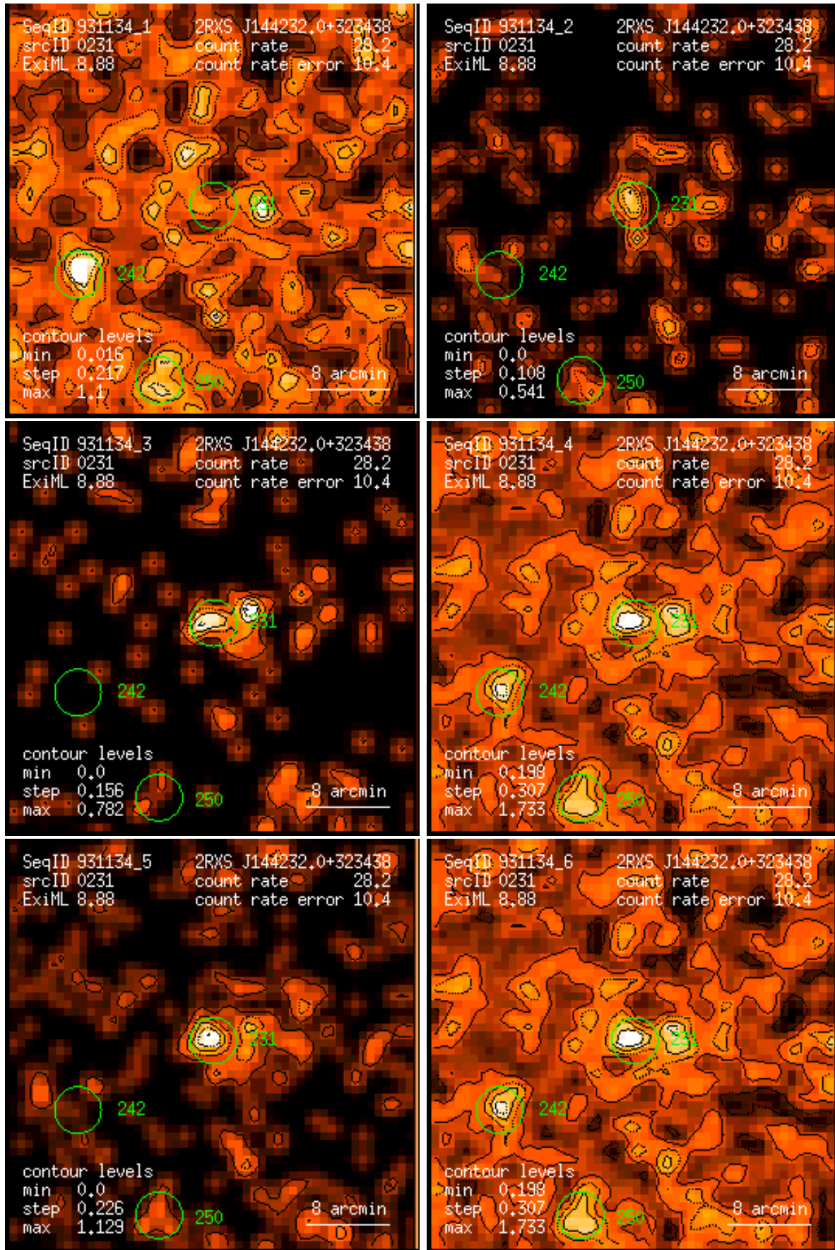
Figure 231: RASS 931134: detection 0231: band rate images, Gaussian filter: (1) PSPC channels 11 – 41, (2) 52 – 90, (3) 91 – 201, (4) 11 – 235, (5) 52 – 201, (6) 11 – 201. Broad band rates in counts/ks. Band rate contour levels in counts/ks/arcmin 2 .
