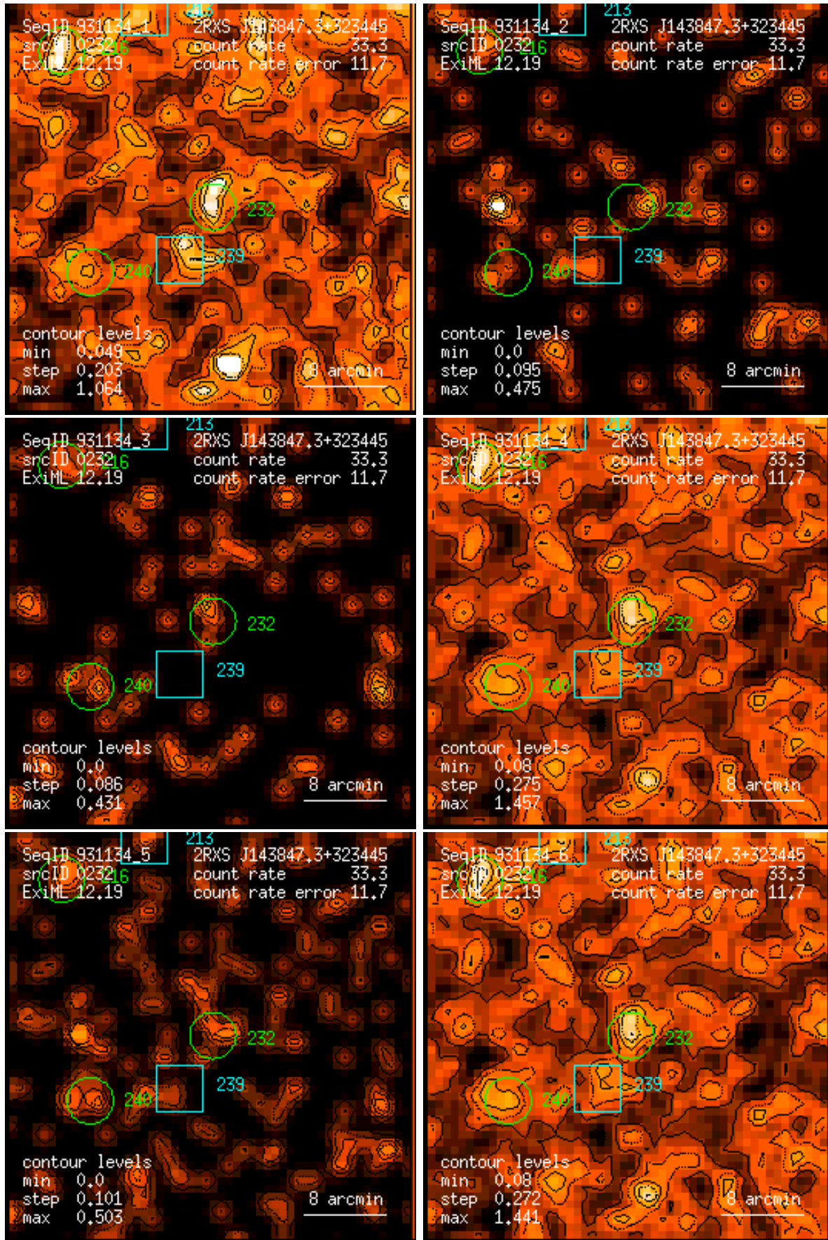
Figure 232: RASS 931134: detection 0232: band rate images, Gaussian filter: (1) PSPC channels 11 – 41, (2) 52 – 90, (3) 91 – 201, (4) 11 – 235, (5) 52 – 201, (6) 11 – 201. Broad band rates in counts/ks. Band rate contour levels in counts/ks/arcmin 2 .
