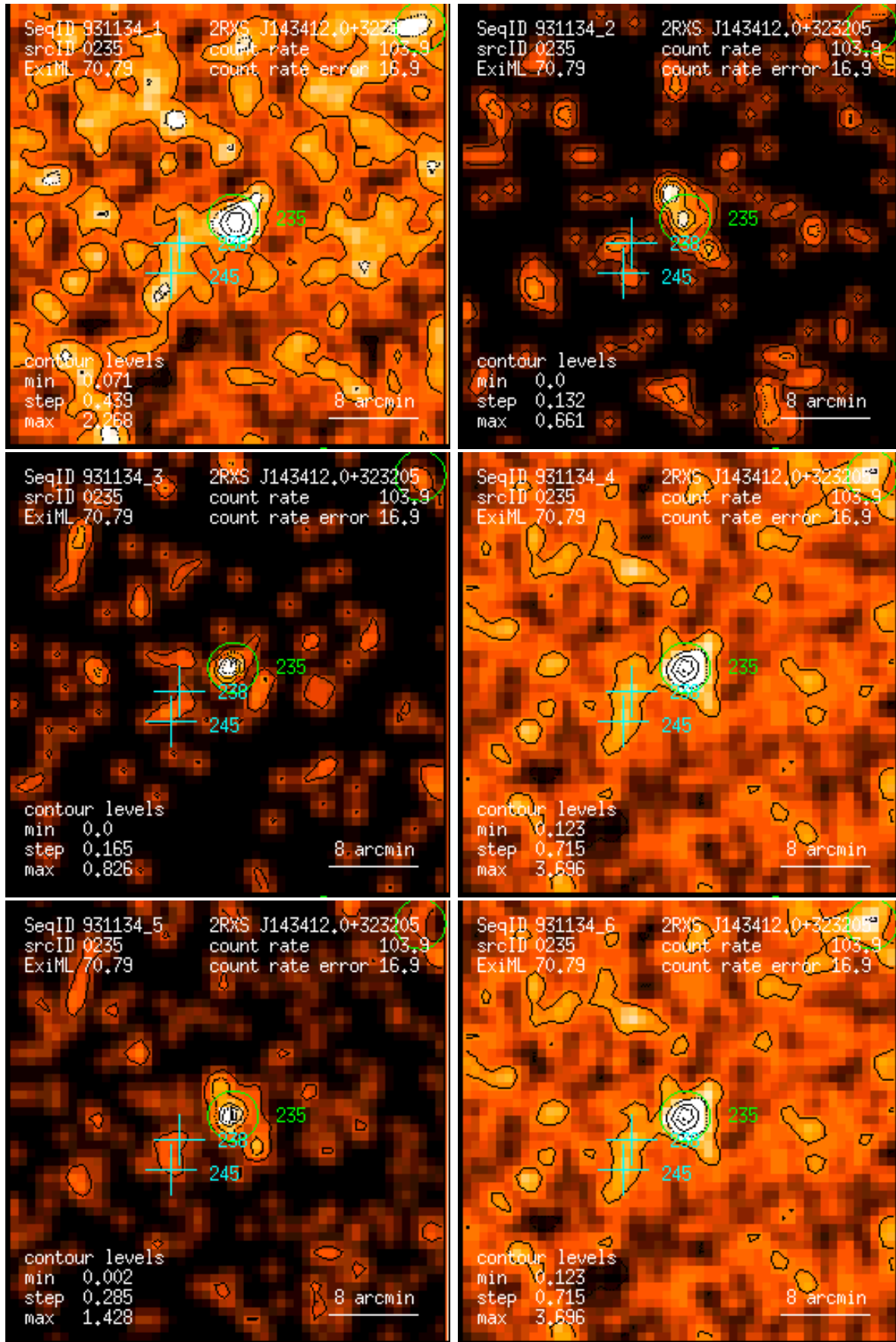
Figure 235: RASS 931134: detection 0235: band rate images, Gaussian filter: (1) PSPC channels 11 – 41, (2) 52 – 90, (3) 91 – 201, (4) 11 – 235, (5) 52 – 201, (6) 11 – 201. Broad band rates in counts/ks. Band rate contour levels in counts/ks/arcmin 2 .
