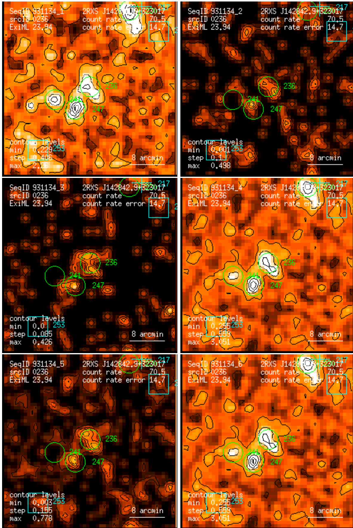
Figure 236: RASS 931134: detection 0236: band rate images, Gaussian filter: (1) PSPC channels 11 – 41, (2) 52 – 90, (3) 91 – 201, (4) 11 – 235, (5) 52 – 201, (6) 11 – 201. Broad band rates in counts/ks. Band rate contour levels in counts/ks/arcmin 2 .
