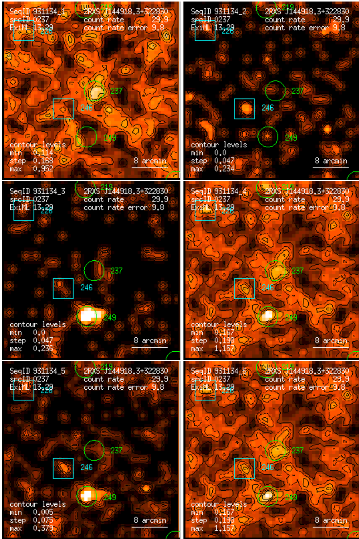
Figure 237: RASS 931134: detection 0237: band rate images, Gaussian filter: (1) PSPC channels 11 – 41, (2) 52 – 90, (3) 91 – 201, (4) 11 – 235, (5) 52 – 201, (6) 11 – 201. Broad band rates in counts/ks. Band rate contour levels in counts/ks/arcmin 2 .
