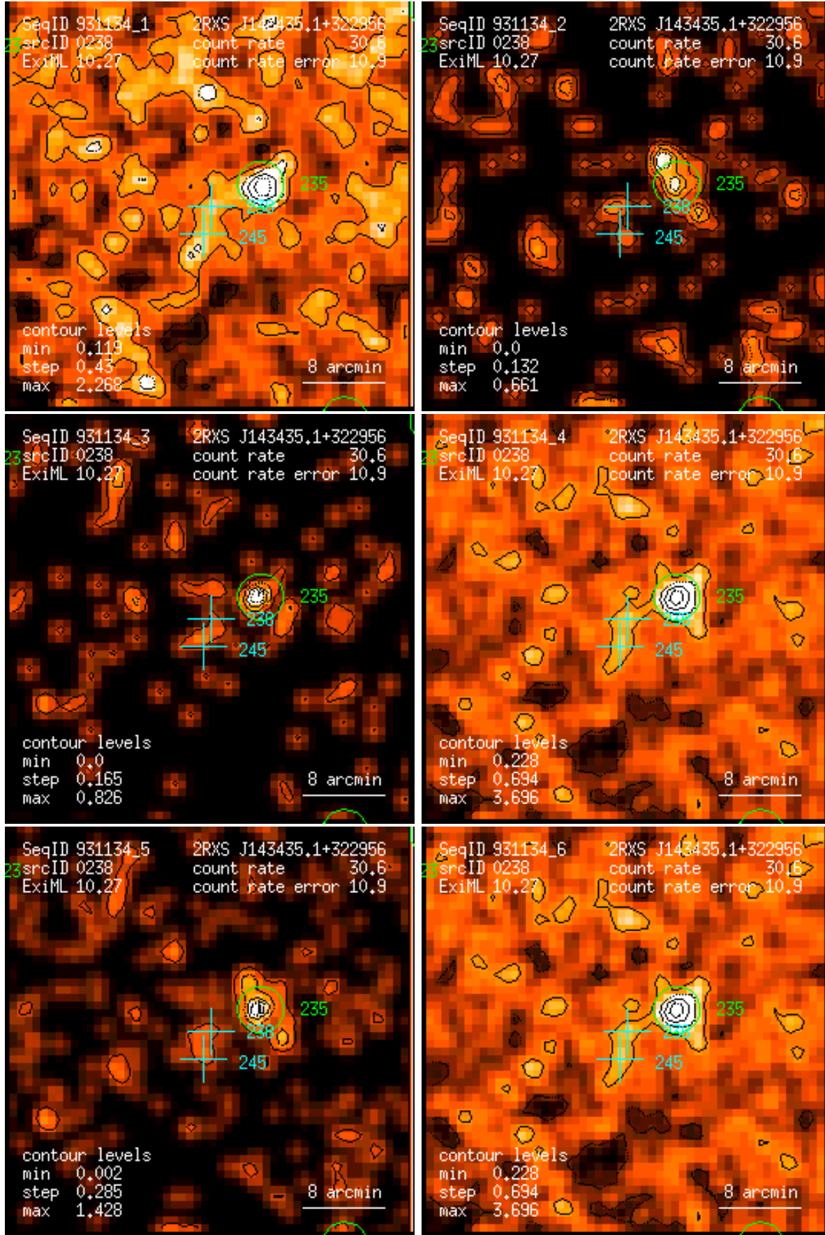
Figure 238: RASS 931134: detection 0238: band rate images, Gaussian filter: (1) PSPC channels 11 – 41, (2) 52 – 90, (3) 91 – 201, (4) 11 – 235, (5) 52 – 201, (6) 11 – 201. Broad band rates in counts/ks. Band rate contour levels in counts/ks/arcmin 2 .
