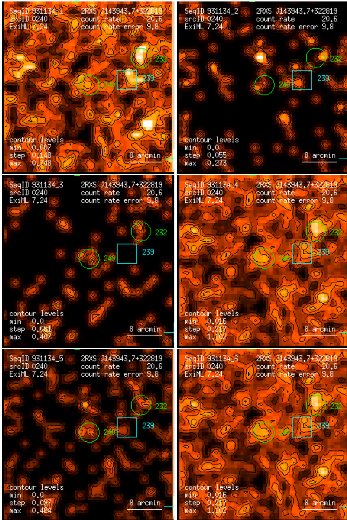
Figure 240: RASS 931134: detection 0240: band rate images, Gaussian filter: (1) PSPC channels 11 – 41, (2) 52 – 90, (3) 91 – 201, (4) 11 – 235, (5) 52 – 201, (6) 11 – 201. Broad band rates in counts/ks. Band rate contour levels in counts/ks/arcmin 2 .
