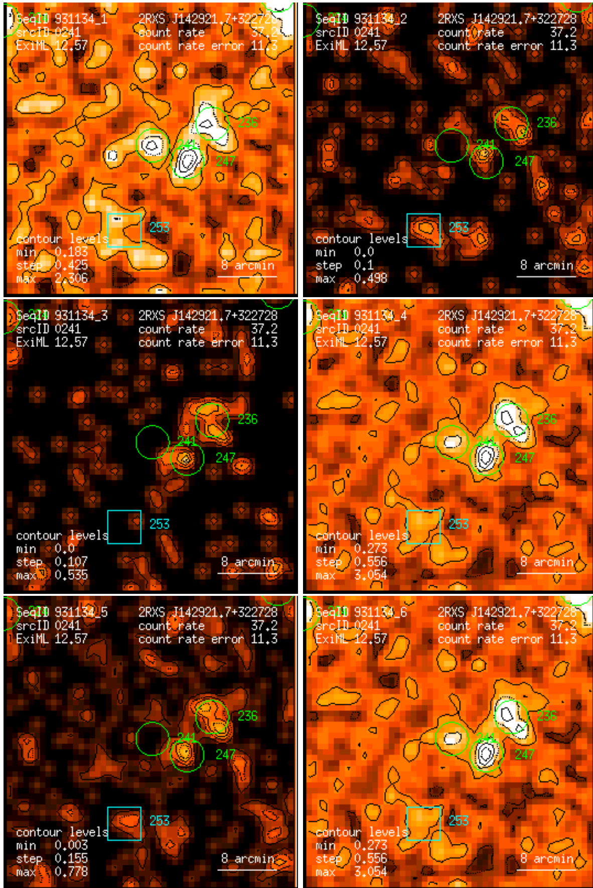
Figure 241: RASS 931134: detection 0241: band rate images, Gaussian filter: (1) PSPC channels 11 – 41, (2) 52 – 90, (3) 91 – 201, (4) 11 – 235, (5) 52 – 201, (6) 11 – 201. Broad band rates in counts/ks. Band rate contour levels in counts/ks/arcmin 2 .
