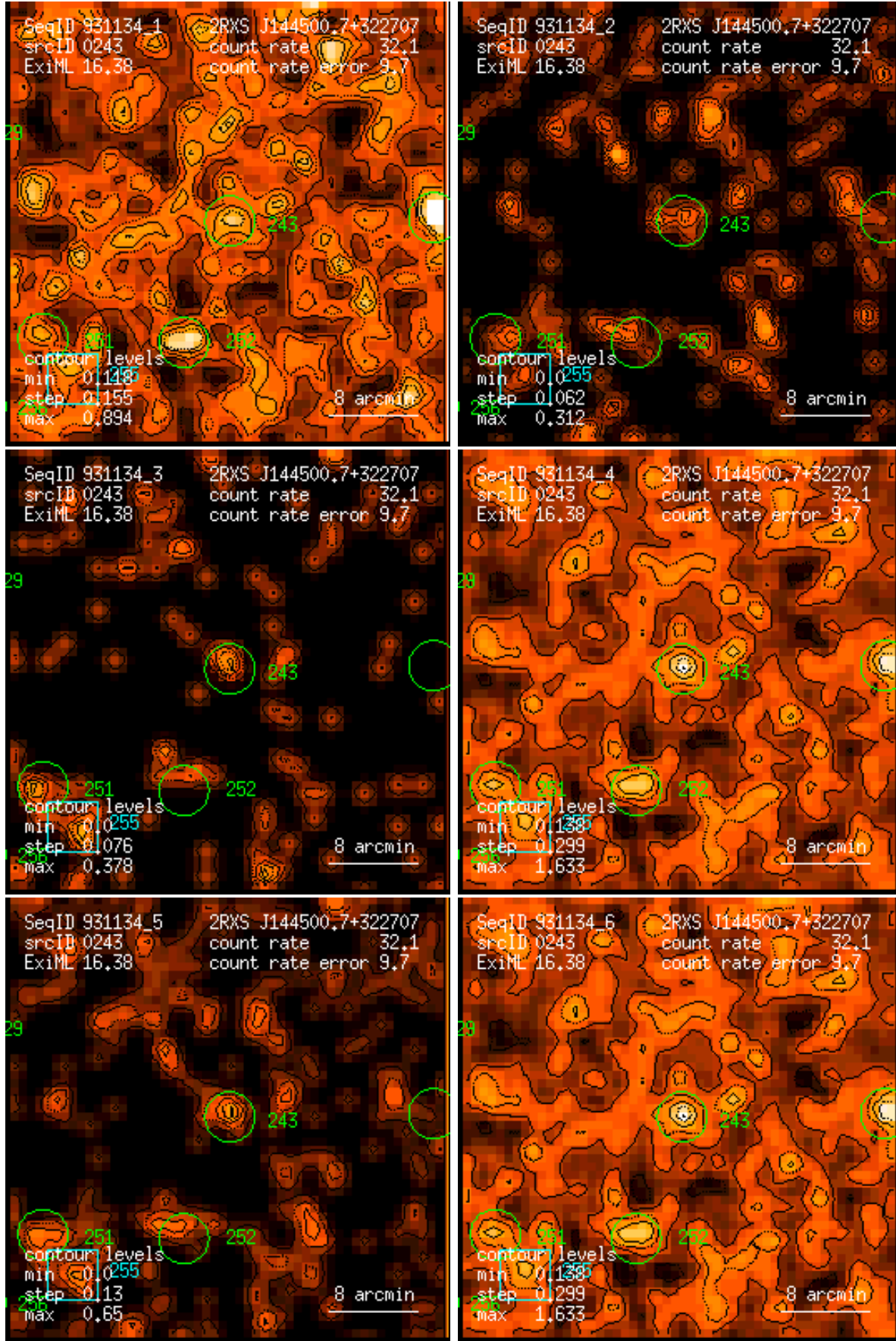
Figure 243: RASS 931134: detection 0243: band rate images, Gaussian filter: (1) PSPC channels 11 – 41, (2) 52 – 90, (3) 91 – 201, (4) 11 – 235, (5) 52 – 201, (6) 11 – 201. Broad band rates in counts/ks. Band rate contour levels in counts/ks/arcmin 2 .
