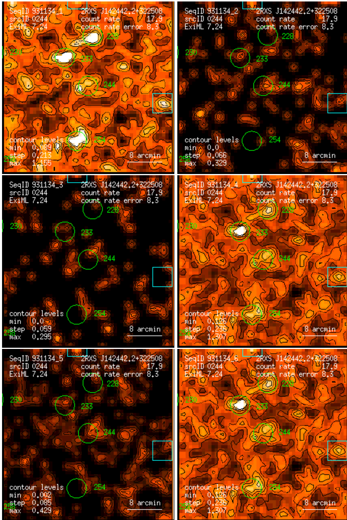
Figure 244: RASS 931134: detection 0244: band rate images, Gaussian filter: (1) PSPC channels 11 – 41, (2) 52 – 90, (3) 91 – 201, (4) 11 – 235, (5) 52 – 201, (6) 11 – 201. Broad band rates in counts/ks. Band rate contour levels in counts/ks/arcmin 2 .
