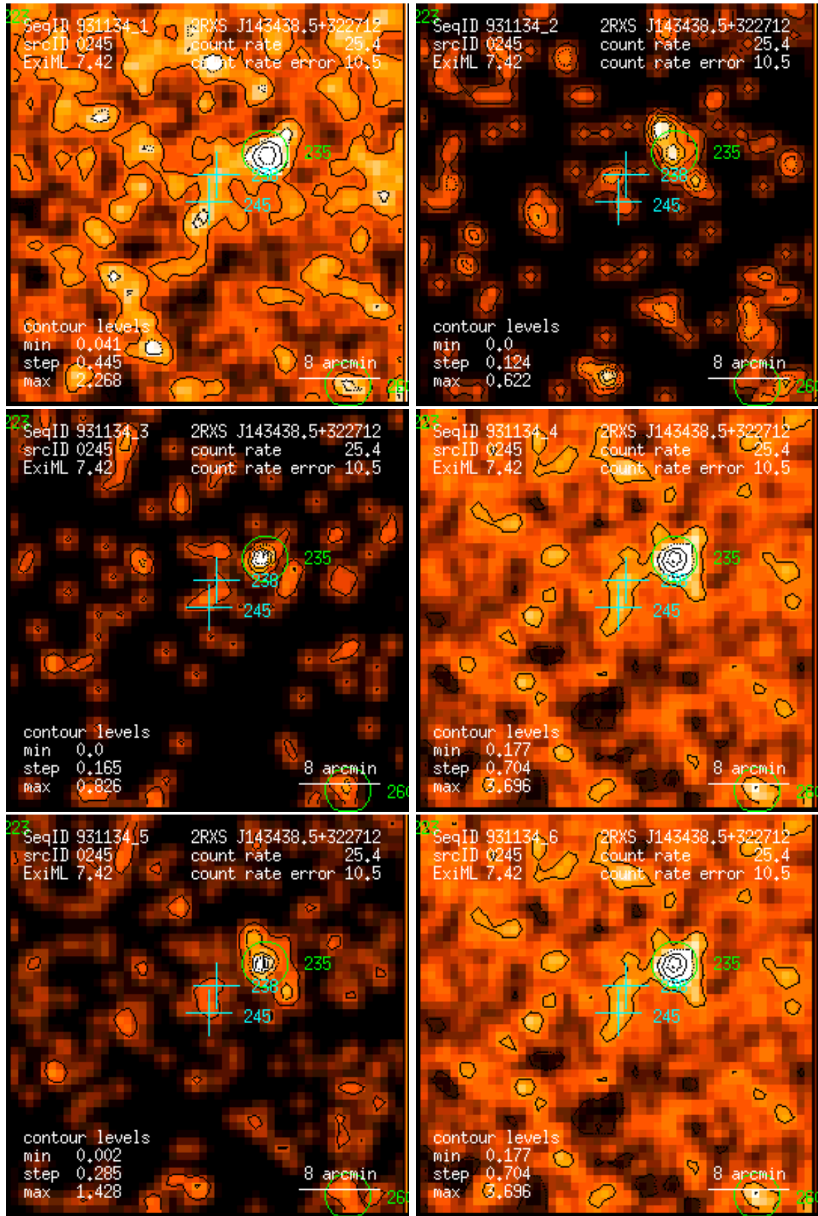
Figure 245: RASS 931134: detection 0245: band rate images, Gaussian filter: (1) PSPC channels 11 – 41, (2) 52 – 90, (3) 91 – 201, (4) 11 – 235, (5) 52 – 201, (6) 11 – 201. Broad band rates in counts/ks. Band rate contour levels in counts/ks/arcmin 2 .
