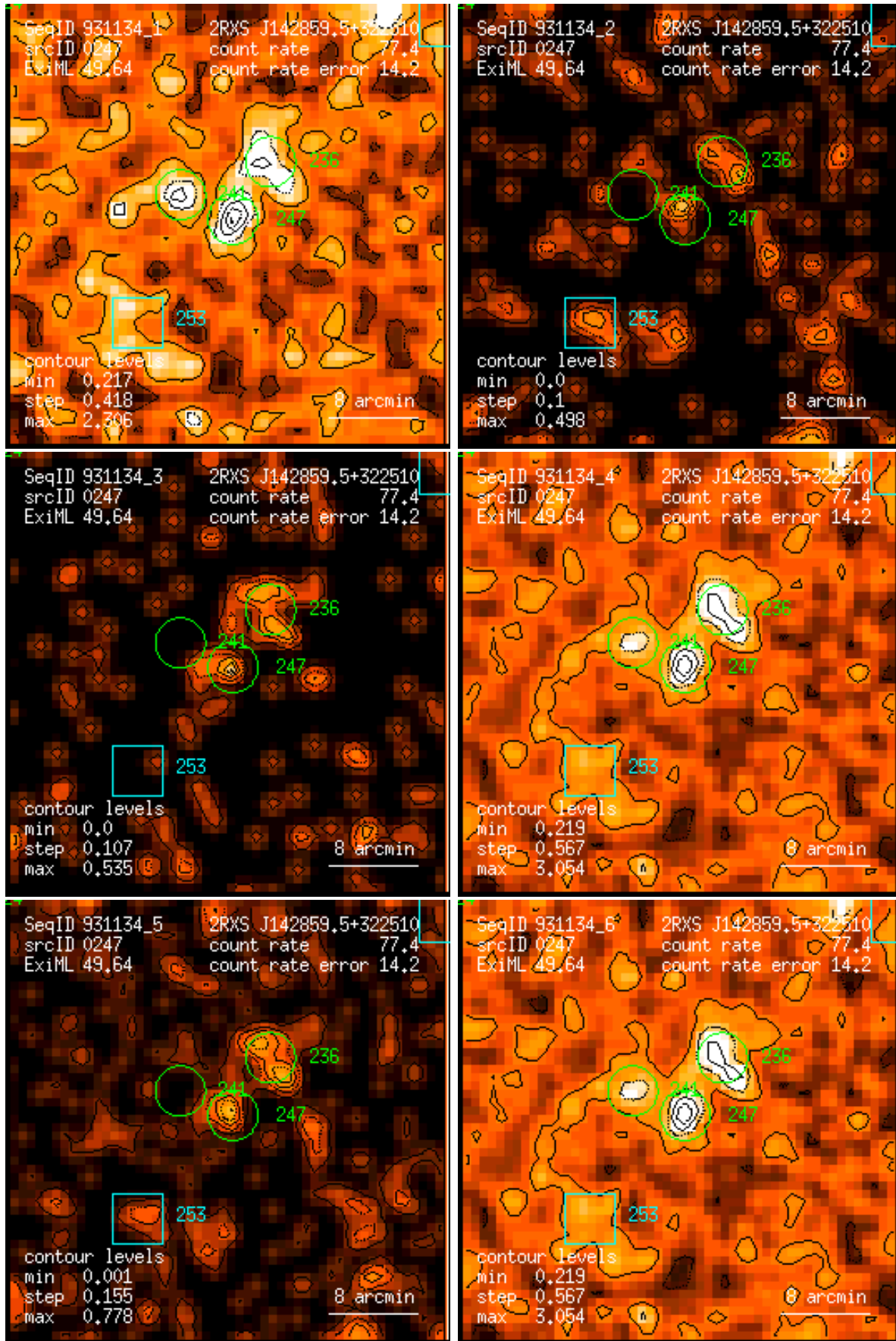
Figure 247: RASS 931134: detection 0247: band rate images, Gaussian filter: (1) PSPC channels 11 – 41, (2) 52 – 90, (3) 91 – 201, (4) 11 – 235, (5) 52 – 201, (6) 11 – 201. Broad band rates in counts/ks. Band rate contour levels in counts/ks/arcmin 2 .
