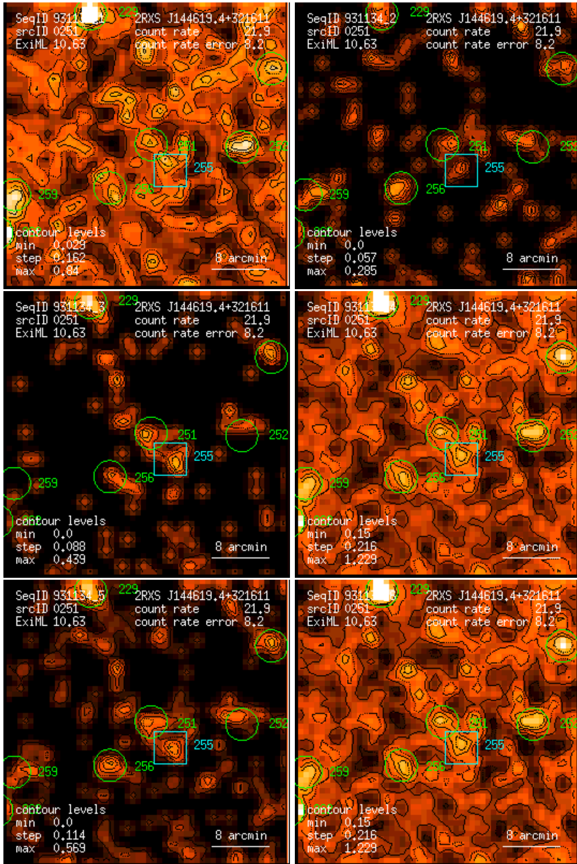
Figure 251: RASS 931134: detection 0251: band rate images, Gaussian filter: (1) PSPC channels 11 – 41, (2) 52 – 90, (3) 91 – 201, (4) 11 – 235, (5) 52 – 201, (6) 11 – 201. Broad band rates in counts/ks. Band rate contour levels in counts/ks/arcmin 2 .
