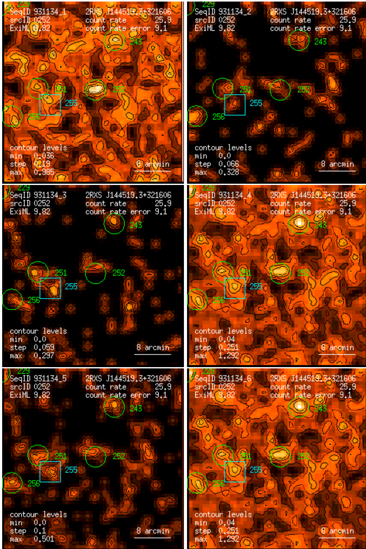
Figure 252: RASS 931134: detection 0252: band rate images, Gaussian filter: (1) PSPC channels 11 – 41, (2) 52 – 90, (3) 91 – 201, (4) 11 – 235, (5) 52 – 201, (6) 11 – 201. Broad band rates in counts/ks. Band rate contour levels in counts/ks/arcmin 2 .
