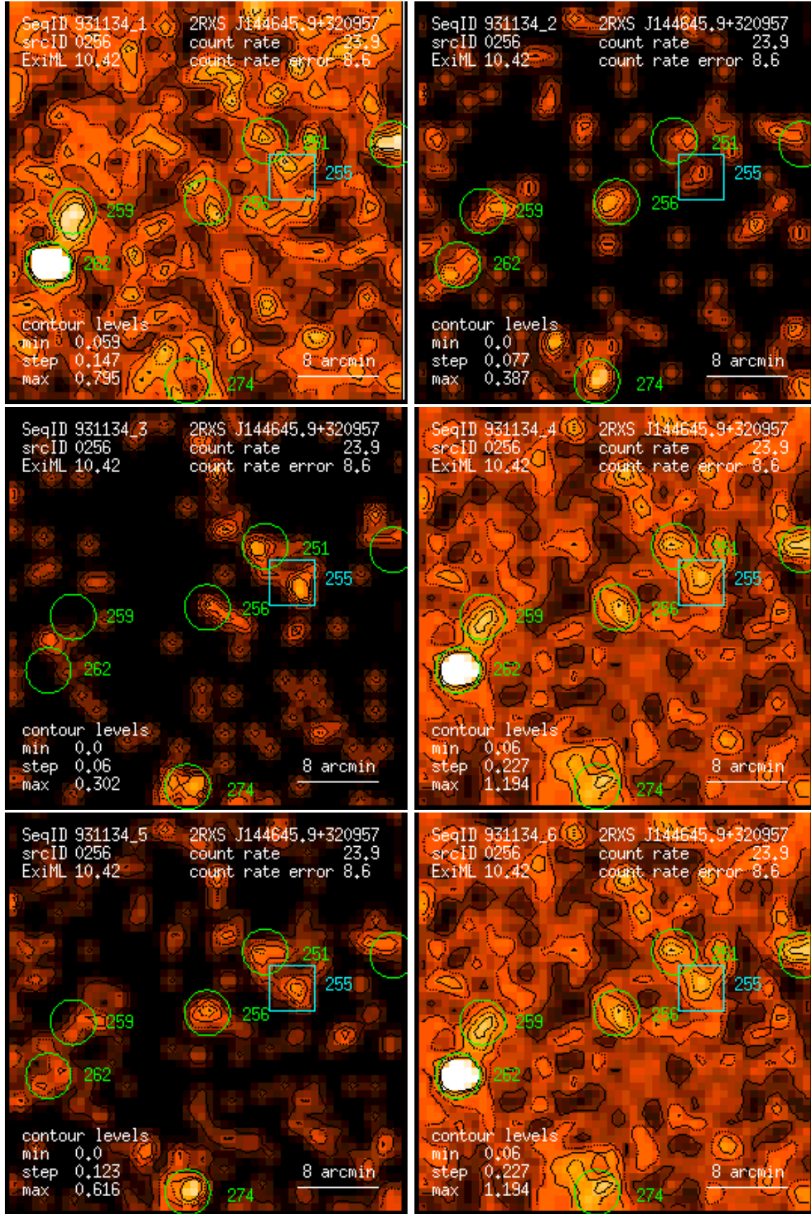
Figure 256: RASS 931134: detection 0256: band rate images, Gaussian filter: (1) PSPC channels 11 – 41, (2) 52 – 90, (3) 91 – 201, (4) 11 – 235, (5) 52 – 201, (6) 11 – 201. Broad band rates in counts/ks. Band rate contour levels in counts/ks/arcmin 2 .
