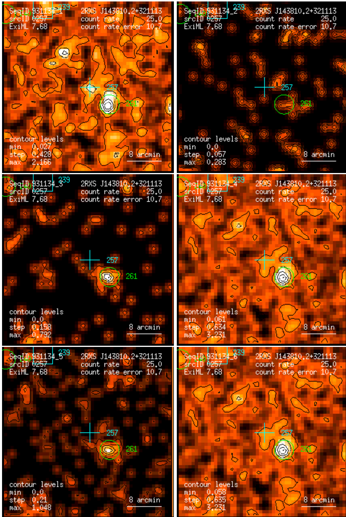
Figure 257: RASS 931134: detection 0257: band rate images, Gaussian filter: (1) PSPC channels 11 – 41, (2) 52 – 90, (3) 91 – 201, (4) 11 – 235, (5) 52 – 201, (6) 11 – 201. Broad band rates in counts/ks. Band rate contour levels in counts/ks/arcmin 2 .
