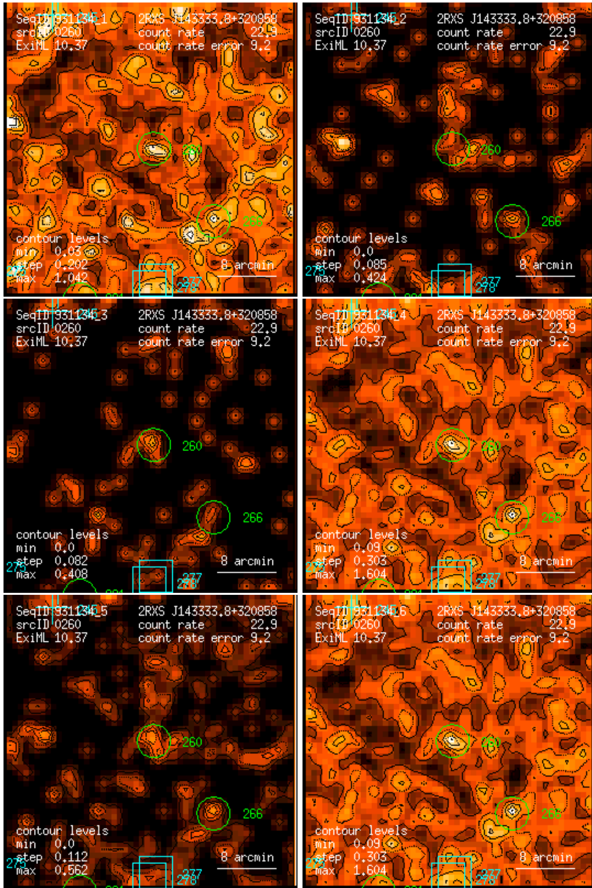
Figure 260: RASS 931134: detection 0260: band rate images, Gaussian filter: (1) PSPC channels 11 – 41, (2) 52 – 90, (3) 91 – 201, (4) 11 – 235, (5) 52 – 201, (6) 11 – 201. Broad band rates in counts/ks. Band rate contour levels in counts/ks/arcmin 2 .
