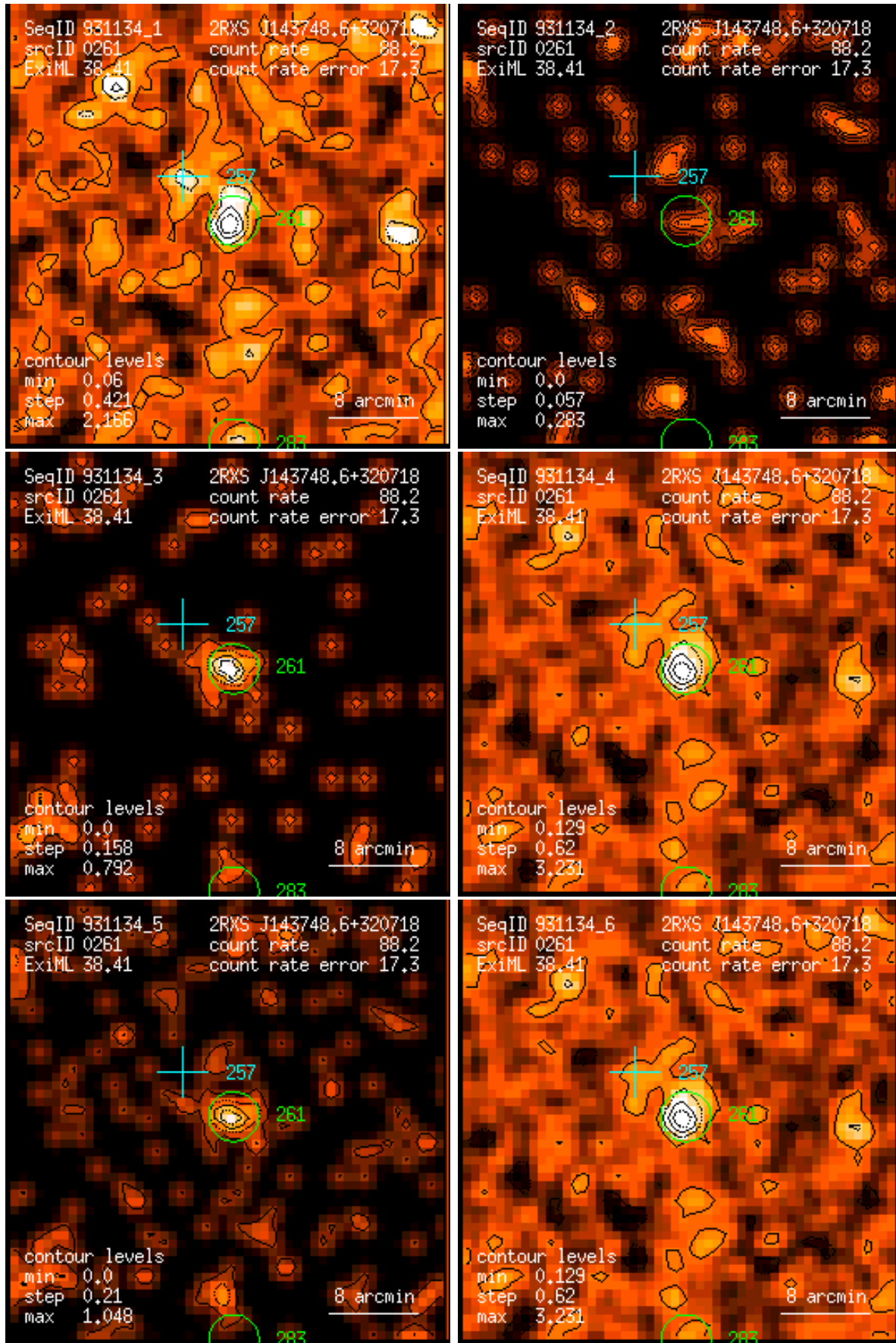
Figure 261: RASS 931134: detection 0261: band rate images, Gaussian filter: (1) PSPC channels 11 – 41, (2) 52 – 90, (3) 91 – 201, (4) 11 – 235, (5) 52 – 201, (6) 11 – 201. Broad band rates in counts/ks. Band rate contour levels in counts/ks/arcmin 2 .
