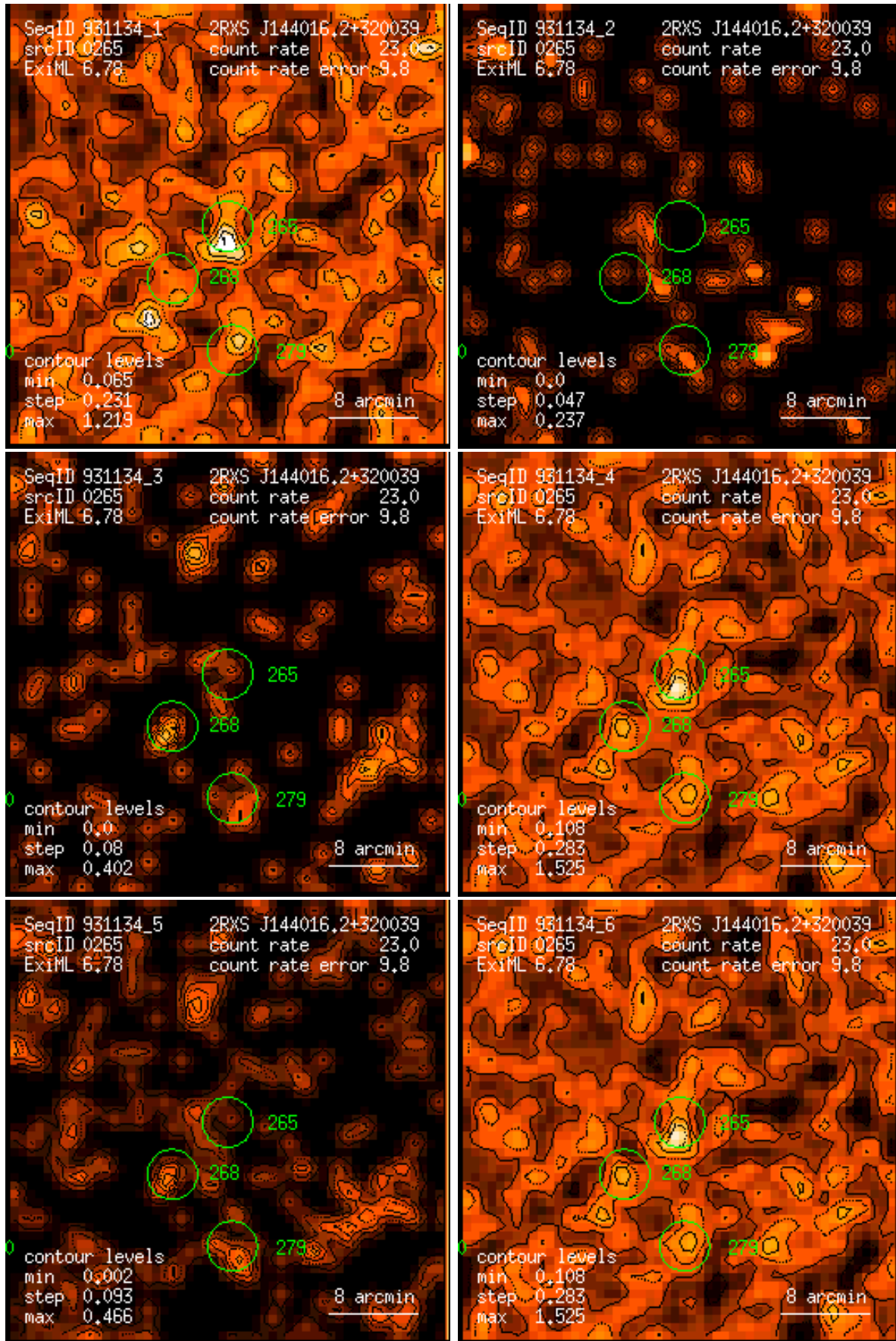
Figure 265: RASS 931134: detection 0265: band rate images, Gaussian filter: (1) PSPC channels 11 – 41, (2) 52 – 90, (3) 91 – 201, (4) 11 – 235, (5) 52 – 201, (6) 11 – 201. Broad band rates in counts/ks. Band rate contour levels in counts/ks/arcmin 2 .
