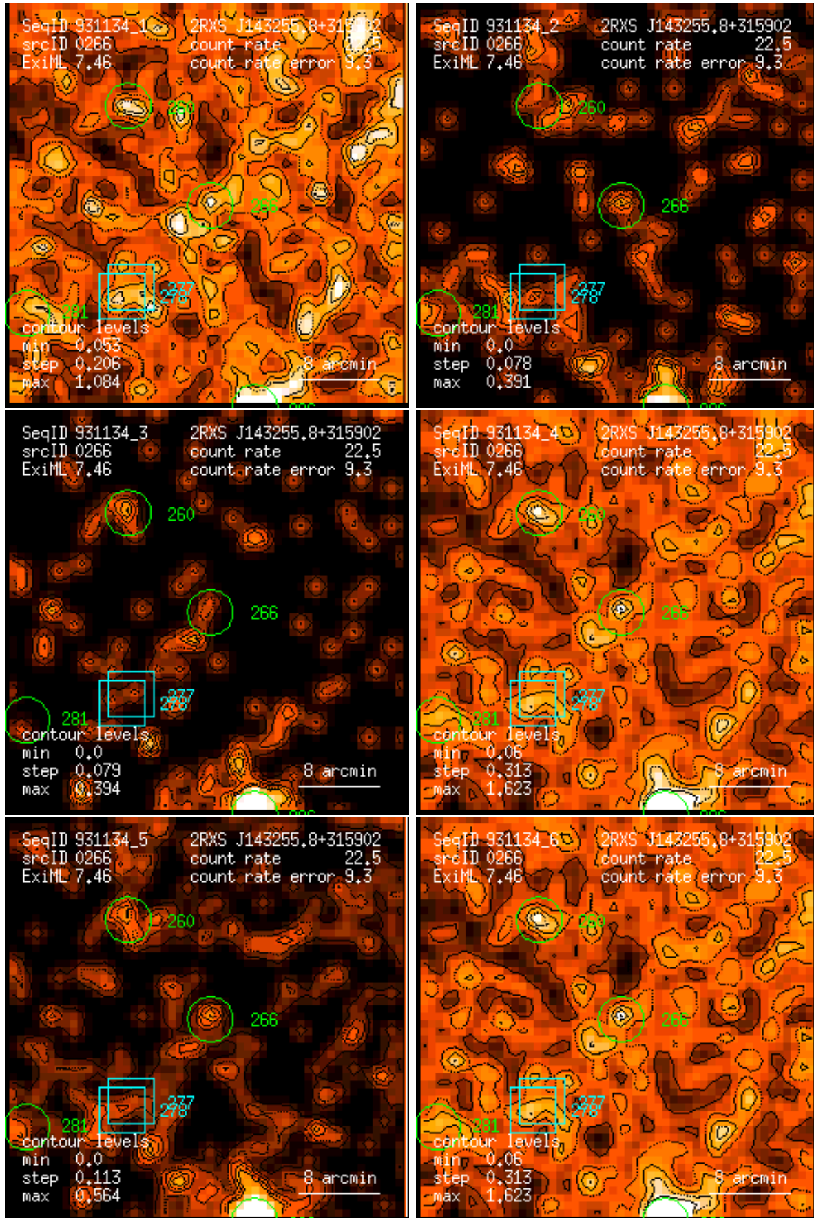
Figure 266: RASS 931134: detection 0266: band rate images, Gaussian filter: (1) PSPC channels 11 – 41, (2) 52 – 90, (3) 91 – 201, (4) 11 – 235, (5) 52 – 201, (6) 11 – 201. Broad band rates in counts/ks. Band rate contour levels in counts/ks/arcmin 2 .
