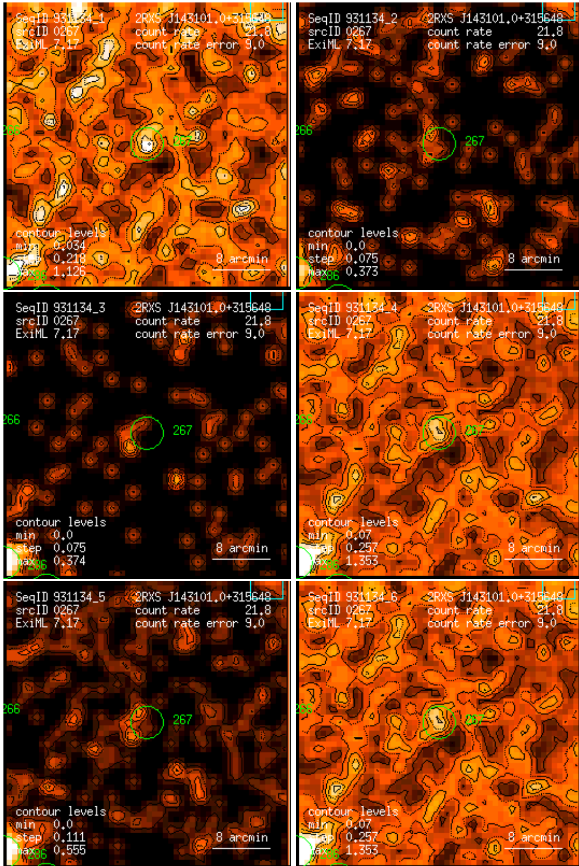
Figure 267: RASS 931134: detection 0267: band rate images, Gaussian filter: (1) PSPC channels 11 – 41, (2) 52 – 90, (3) 91 – 201, (4) 11 – 235, (5) 52 – 201, (6) 11 – 201. Broad band rates in counts/ks. Band rate contour levels in counts/ks/arcmin 2 .
