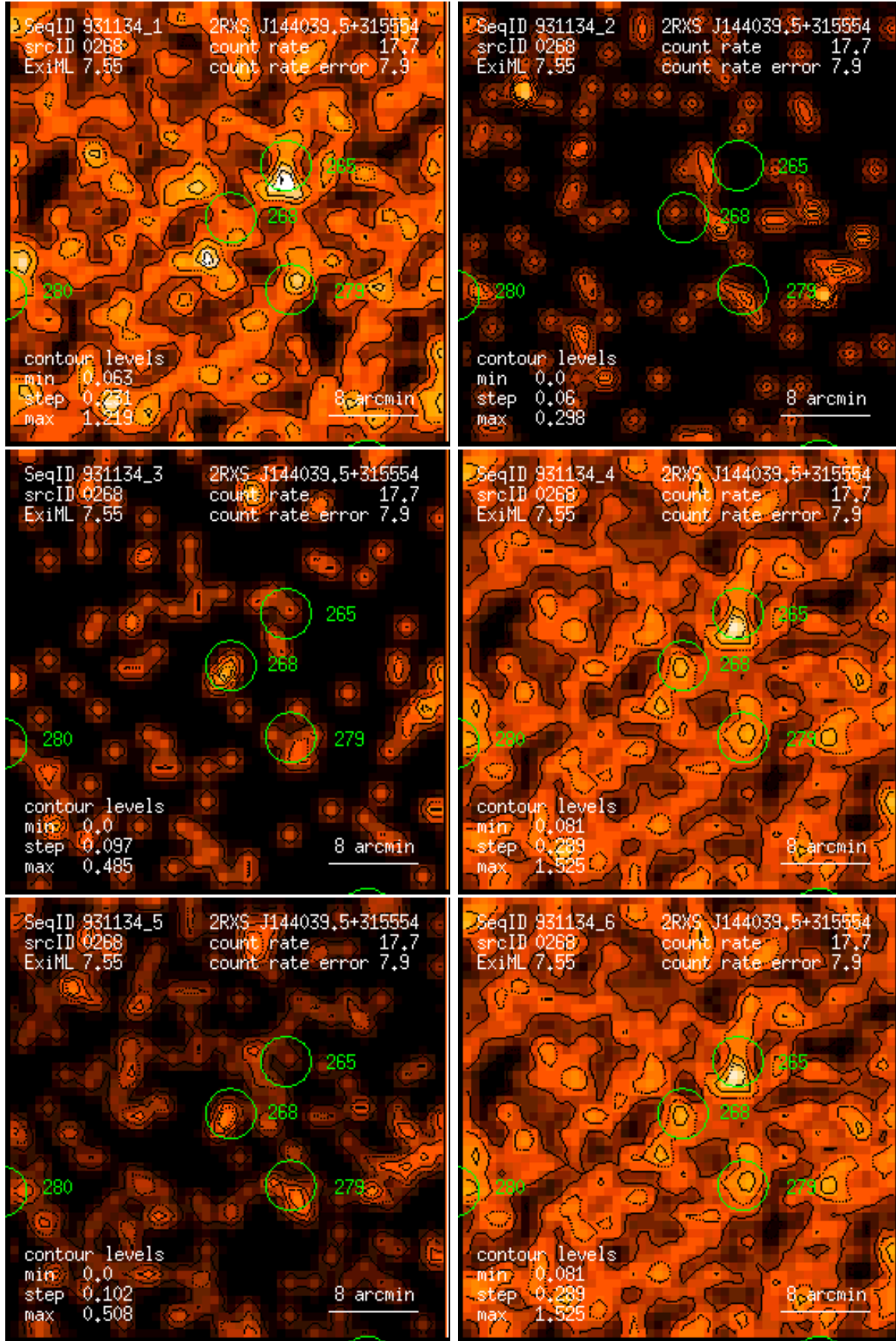
Figure 268: RASS 931134: detection 0268: band rate images, Gaussian filter: (1) PSPC channels 11 – 41, (2) 52 – 90, (3) 91 – 201, (4) 11 – 235, (5) 52 – 201, (6) 11 – 201. Broad band rates in counts/ks. Band rate contour levels in counts/ks/arcmin 2 .
