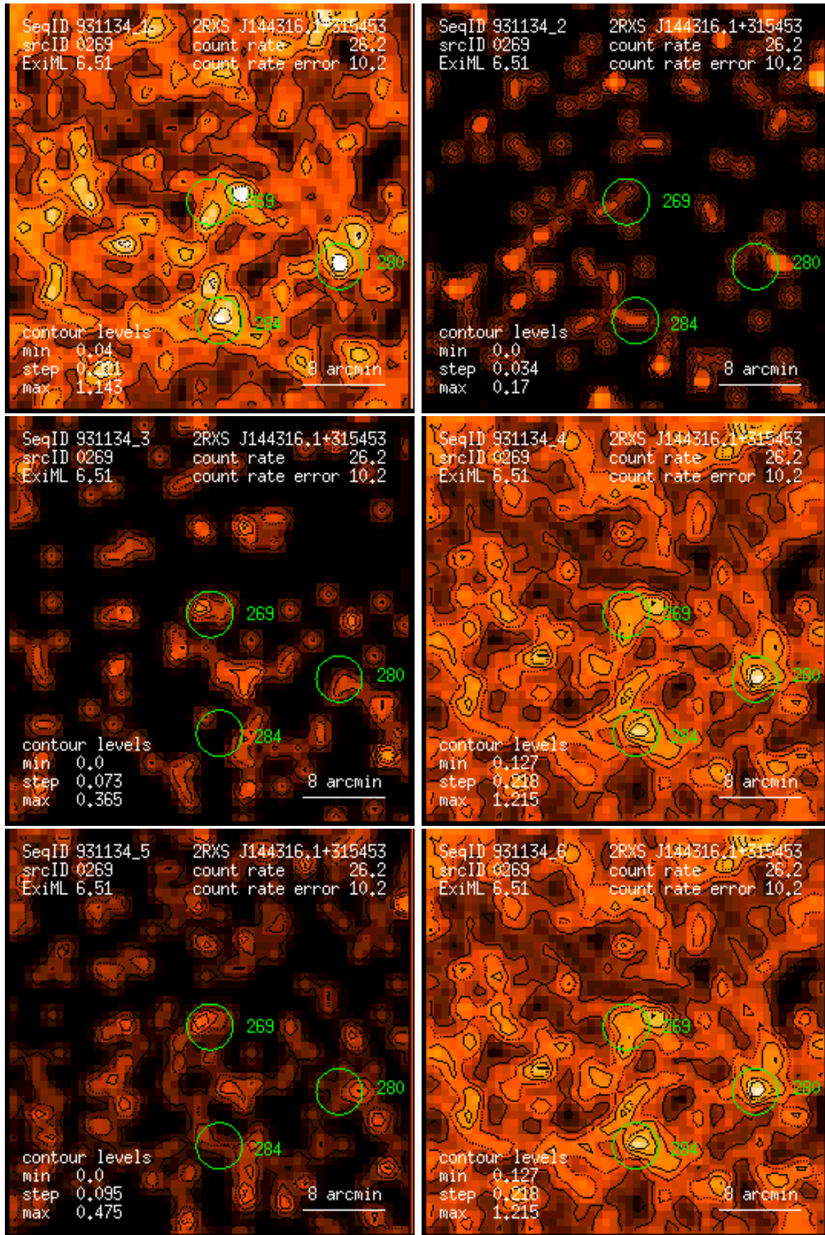
Figure 269: RASS 931134: detection 0269: band rate images, Gaussian filter: (1) PSPC channels 11 – 41, (2) 52 – 90, (3) 91 – 201, (4) 11 – 235, (5) 52 – 201, (6) 11 – 201. Broad band rates in counts/ks. Band rate contour levels in counts/ks/arcmin 2 .
