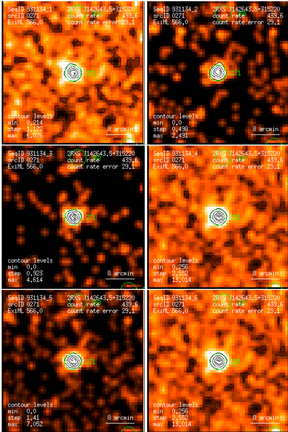
Figure 271: RASS 931134: detection 0271: band rate images, Gaussian filter: (1) PSPC channels 11 – 41, (2) 52 – 90, (3) 91 – 201, (4) 11 – 235, (5) 52 – 201, (6) 11 – 201. Broad band rates in counts/ks. Band rate contour levels in counts/ks/arcmin 2 .
