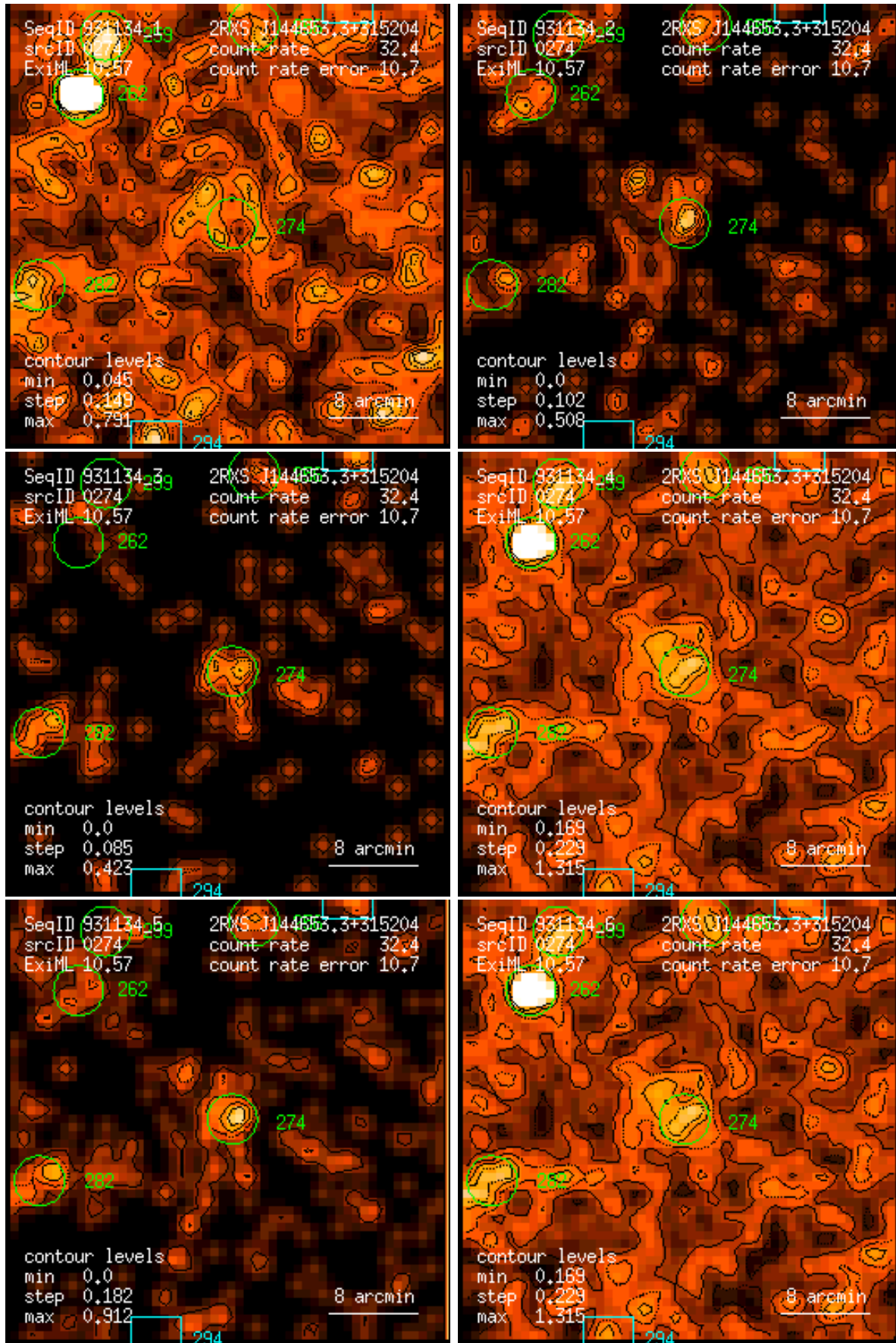
Figure 274: RASS 931134: detection 0274: band rate images, Gaussian filter: (1) PSPC channels 11 – 41, (2) 52 – 90, (3) 91 – 201, (4) 11 – 235, (5) 52 – 201, (6) 11 – 201. Broad band rates in counts/ks. Band rate contour levels in counts/ks/arcmin 2 .
