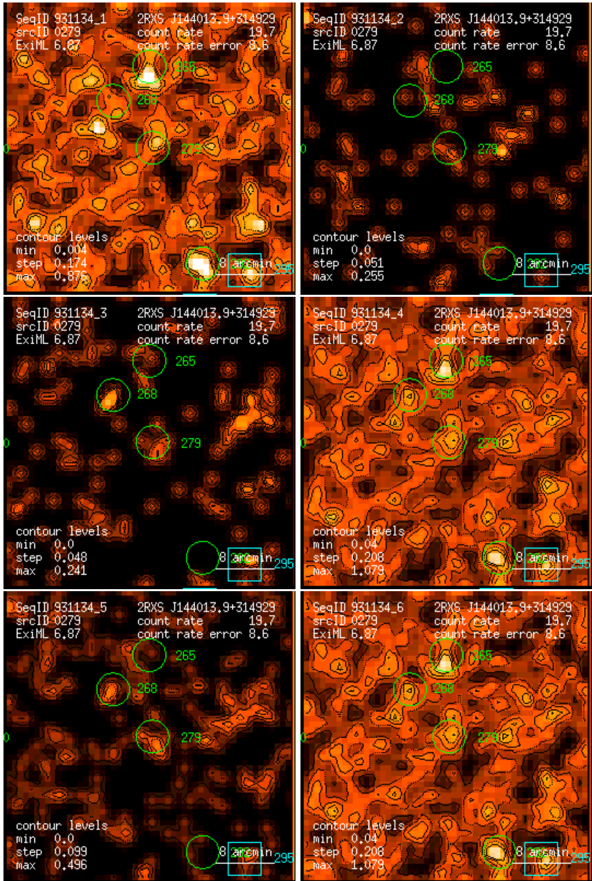
Figure 279: RASS 931134: detection 0279: band rate images, Gaussian filter: (1) PSPC channels 11 – 41, (2) 52 – 90, (3) 91 – 201, (4) 11 – 235, (5) 52 – 201, (6) 11 – 201. Broad band rates in counts/ks. Band rate contour levels in counts/ks/arcmin 2 .
