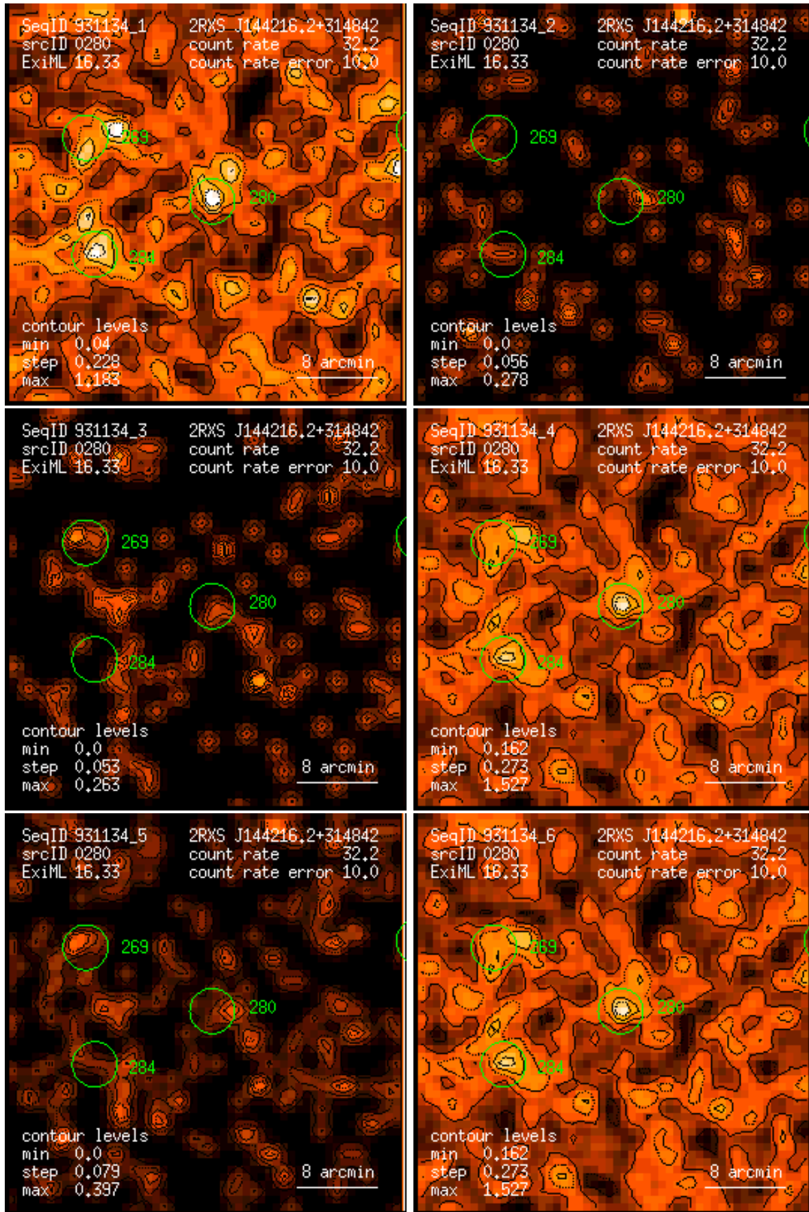
Figure 280: RASS 931134: detection 0280: band rate images, Gaussian filter: (1) PSPC channels 11 – 41, (2) 52 – 90, (3) 91 – 201, (4) 11 – 235, (5) 52 – 201, (6) 11 – 201. Broad band rates in counts/ks. Band rate contour levels in counts/ks/arcmin 2 .
