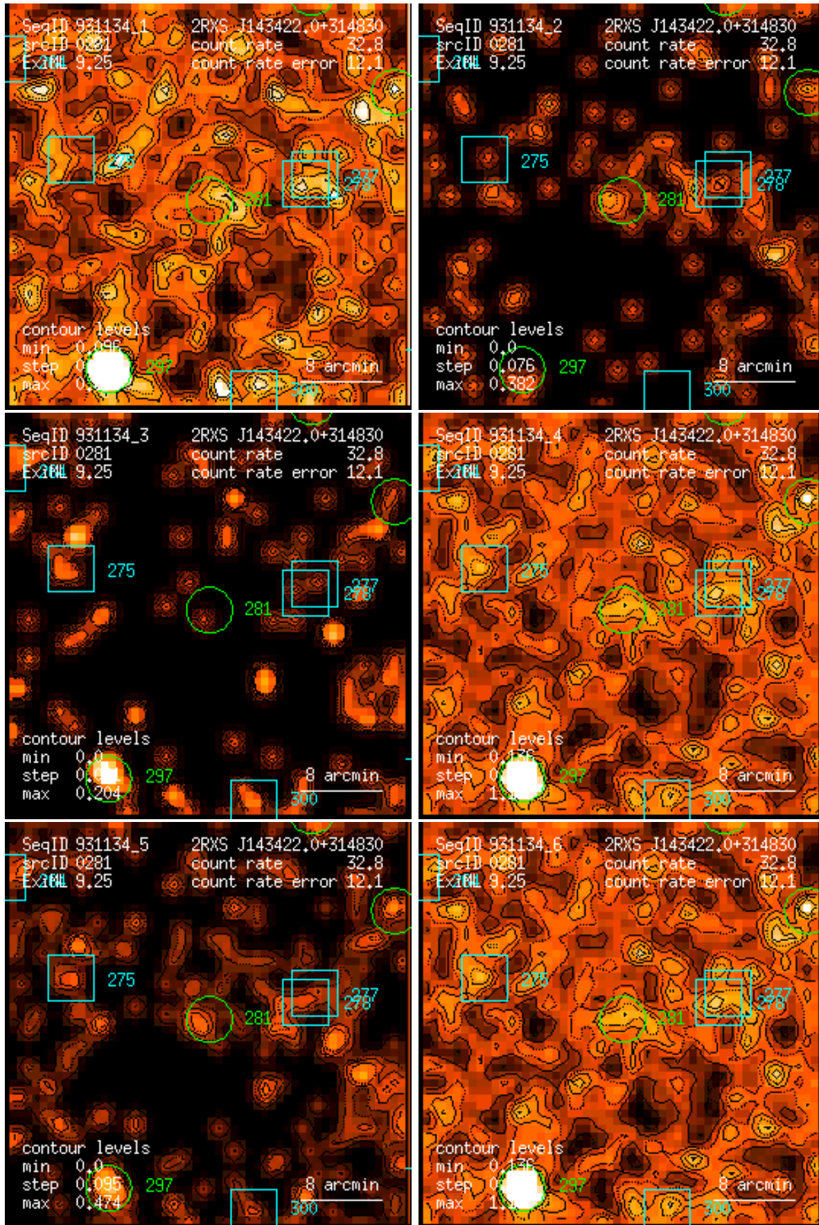
Figure 281: RASS 931134: detection 0281: band rate images, Gaussian filter: (1) PSPC channels 11 – 41, (2) 52 – 90, (3) 91 – 201, (4) 11 – 235, (5) 52 – 201, (6) 11 – 201. Broad band rates in counts/ks. Band rate contour levels in counts/ks/arcmin 2 .
