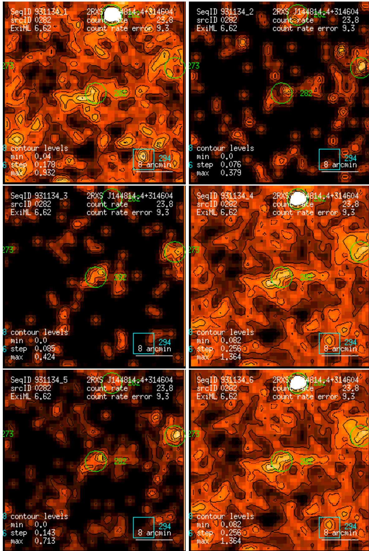
Figure 282: RASS 931134: detection 0282: band rate images, Gaussian filter: (1) PSPC channels 11 – 41, (2) 52 – 90, (3) 91 – 201, (4) 11 – 235, (5) 52 – 201, (6) 11 – 201. Broad band rates in counts/ks. Band rate contour levels in counts/ks/arcmin 2 .
