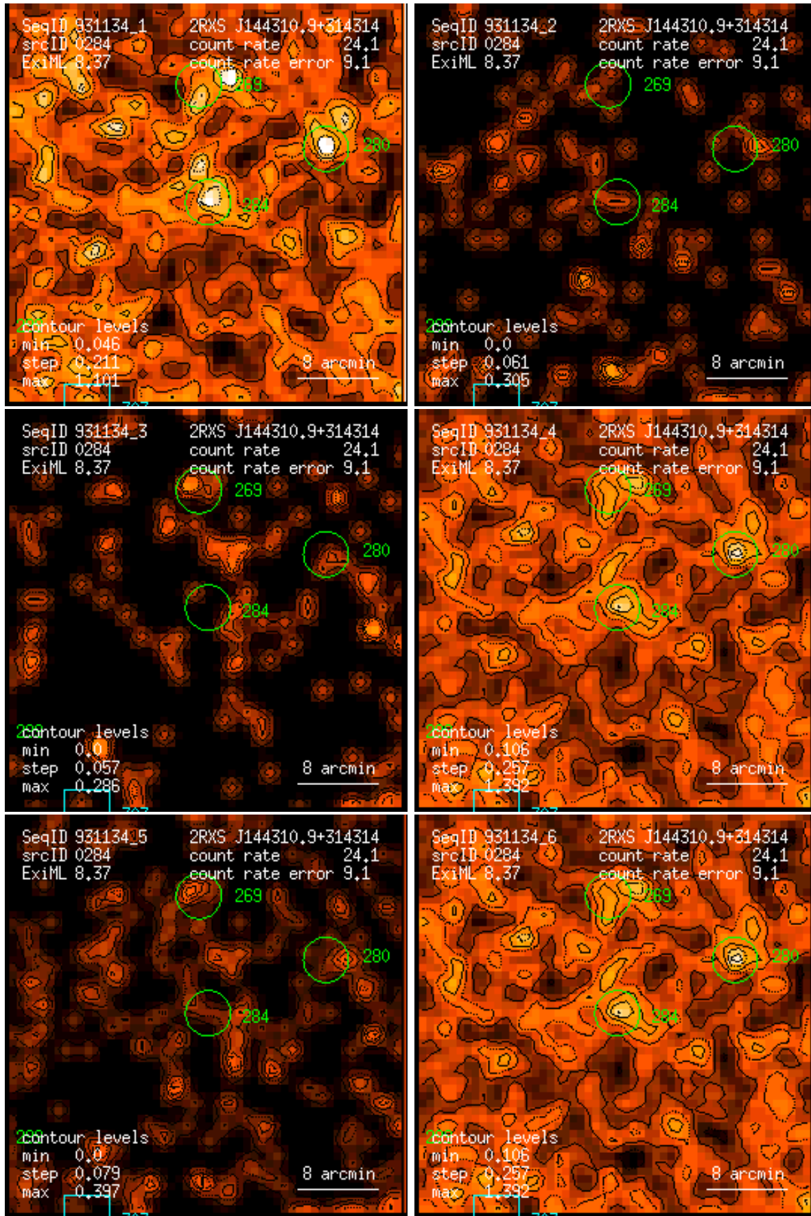
Figure 284: RASS 931134: detection 0284: band rate images, Gaussian filter: (1) PSPC channels 11 – 41, (2) 52 – 90, (3) 91 – 201, (4) 11 – 235, (5) 52 – 201, (6) 11 – 201. Broad band rates in counts/ks. Band rate contour levels in counts/ks/arcmin 2 .
