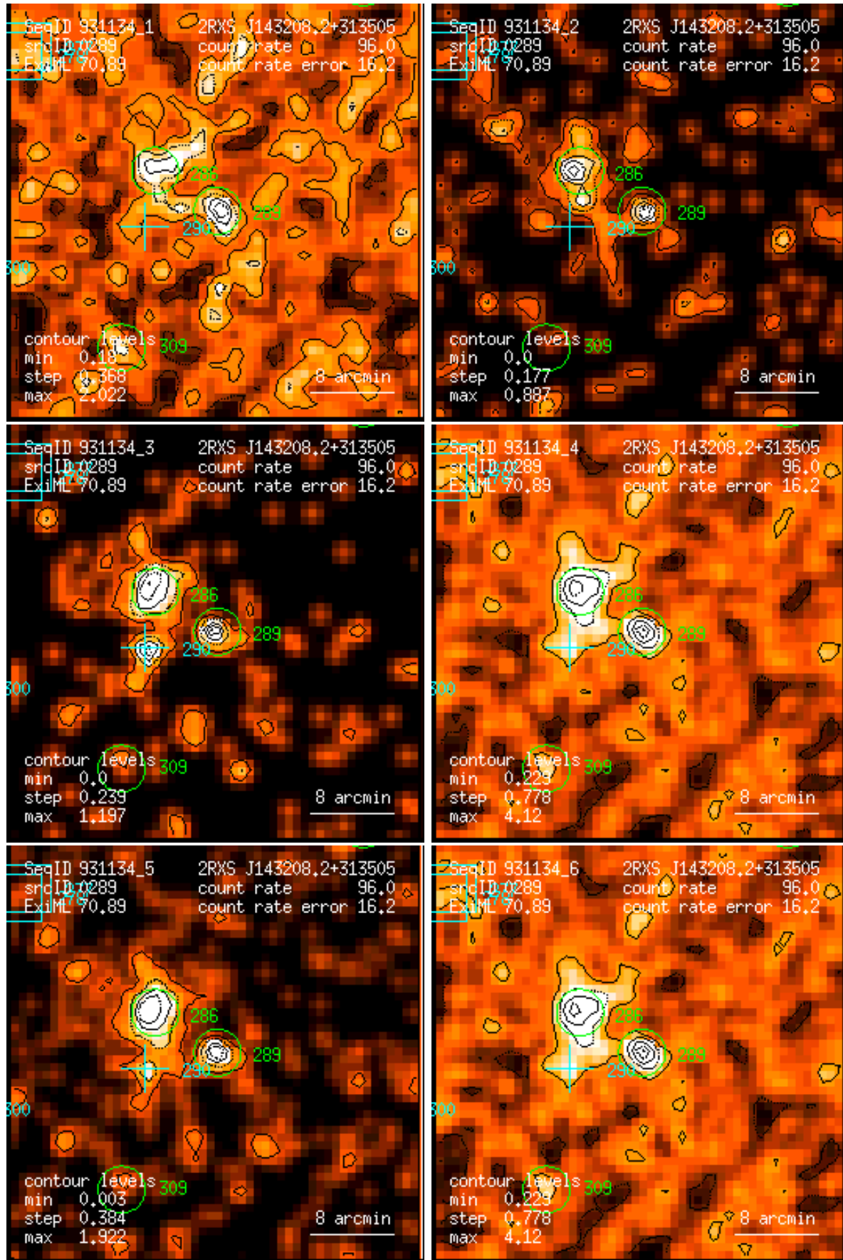
Figure 289: RASS 931134: detection 0289: band rate images, Gaussian filter: (1) PSPC channels 11 – 41, (2) 52 – 90, (3) 91 – 201, (4) 11 – 235, (5) 52 – 201, (6) 11 – 201. Broad band rates in counts/ks. Band rate contour levels in counts/ks/arcmin 2 .
