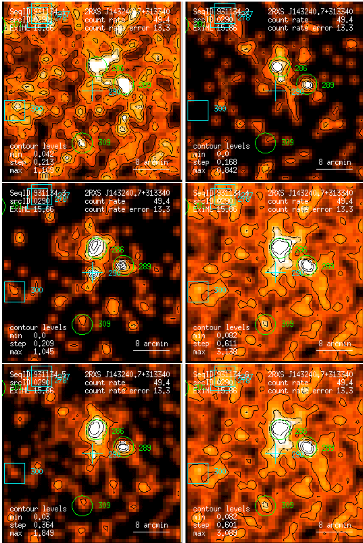
Figure 290: RASS 931134: detection 0290: band rate images, Gaussian filter: (1) PSPC channels 11 – 41, (2) 52 – 90, (3) 91 – 201, (4) 11 – 235, (5) 52 – 201, (6) 11 – 201. Broad band rates in counts/ks. Band rate contour levels in counts/ks/arcmin 2 .
