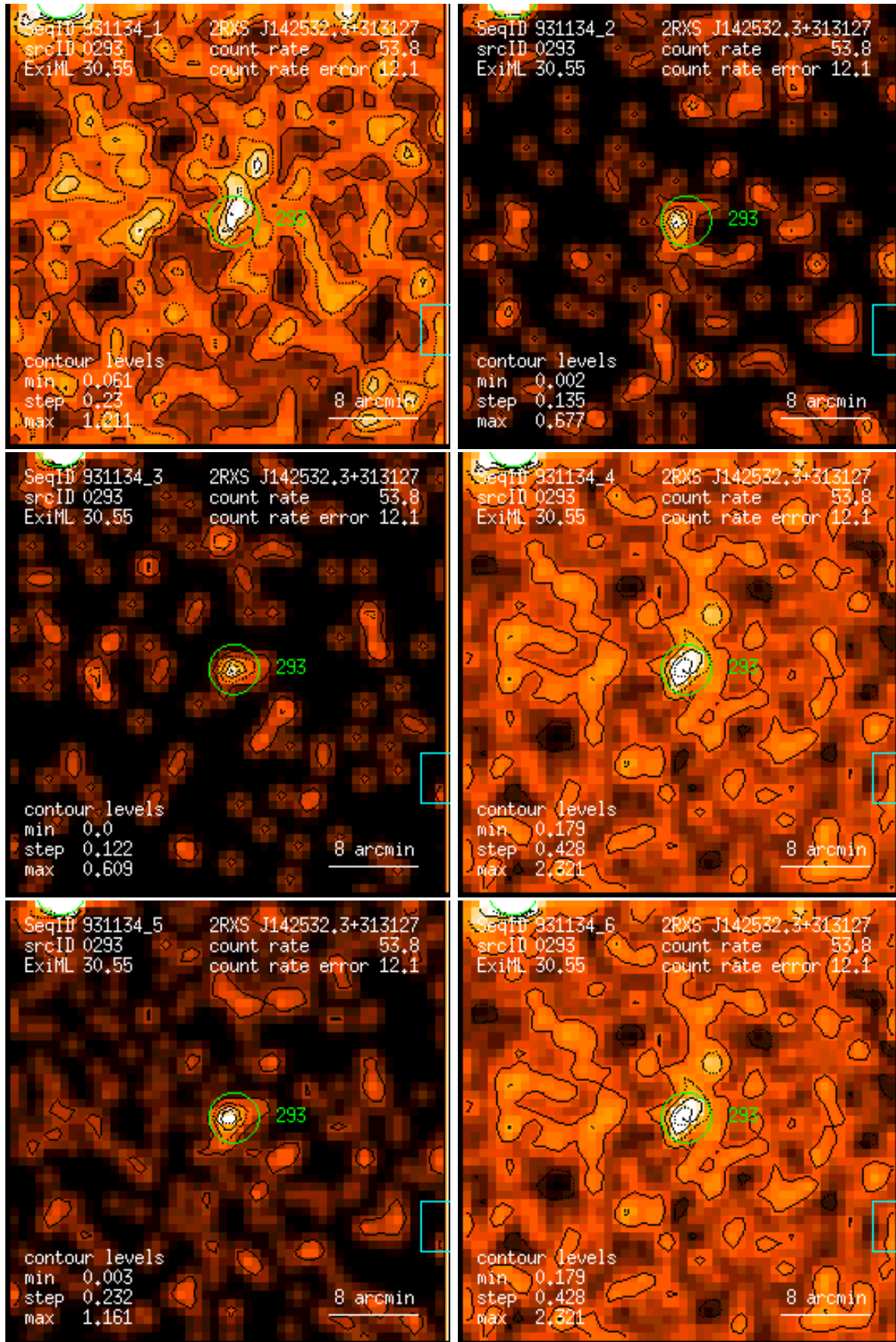
Figure 293: RASS 931134: detection 0293: band rate images, Gaussian filter: (1) PSPC channels 11 – 41, (2) 52 – 90, (3) 91 – 201, (4) 11 – 235, (5) 52 – 201, (6) 11 – 201. Broad band rates in counts/ks. Band rate contour levels in counts/ks/arcmin 2 .
