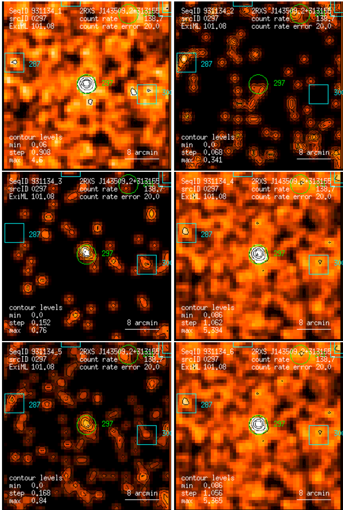
Figure 297: RASS 931134: detection 0297: band rate images, Gaussian filter: (1) PSPC channels 11 – 41, (2) 52 – 90, (3) 91 – 201, (4) 11 – 235, (5) 52 – 201, (6) 11 – 201. Broad band rates in counts/ks. Band rate contour levels in counts/ks/arcmin 2 .
