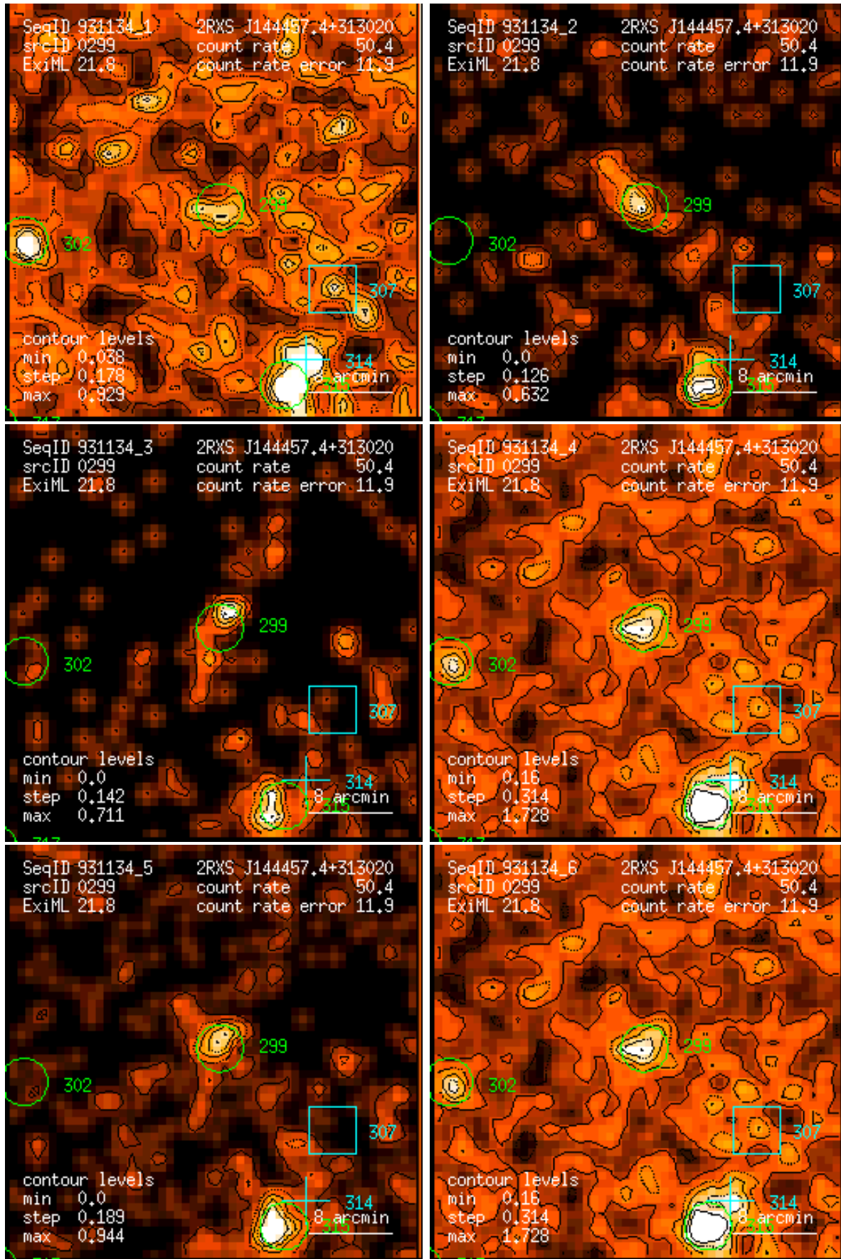
Figure 299: RASS 931134: detection 0299: band rate images, Gaussian filter: (1) PSPC channels 11 – 41, (2) 52 – 90, (3) 91 – 201, (4) 11 – 235, (5) 52 – 201, (6) 11 – 201. Broad band rates in counts/ks. Band rate contour levels in counts/ks/arcmin 2 .
