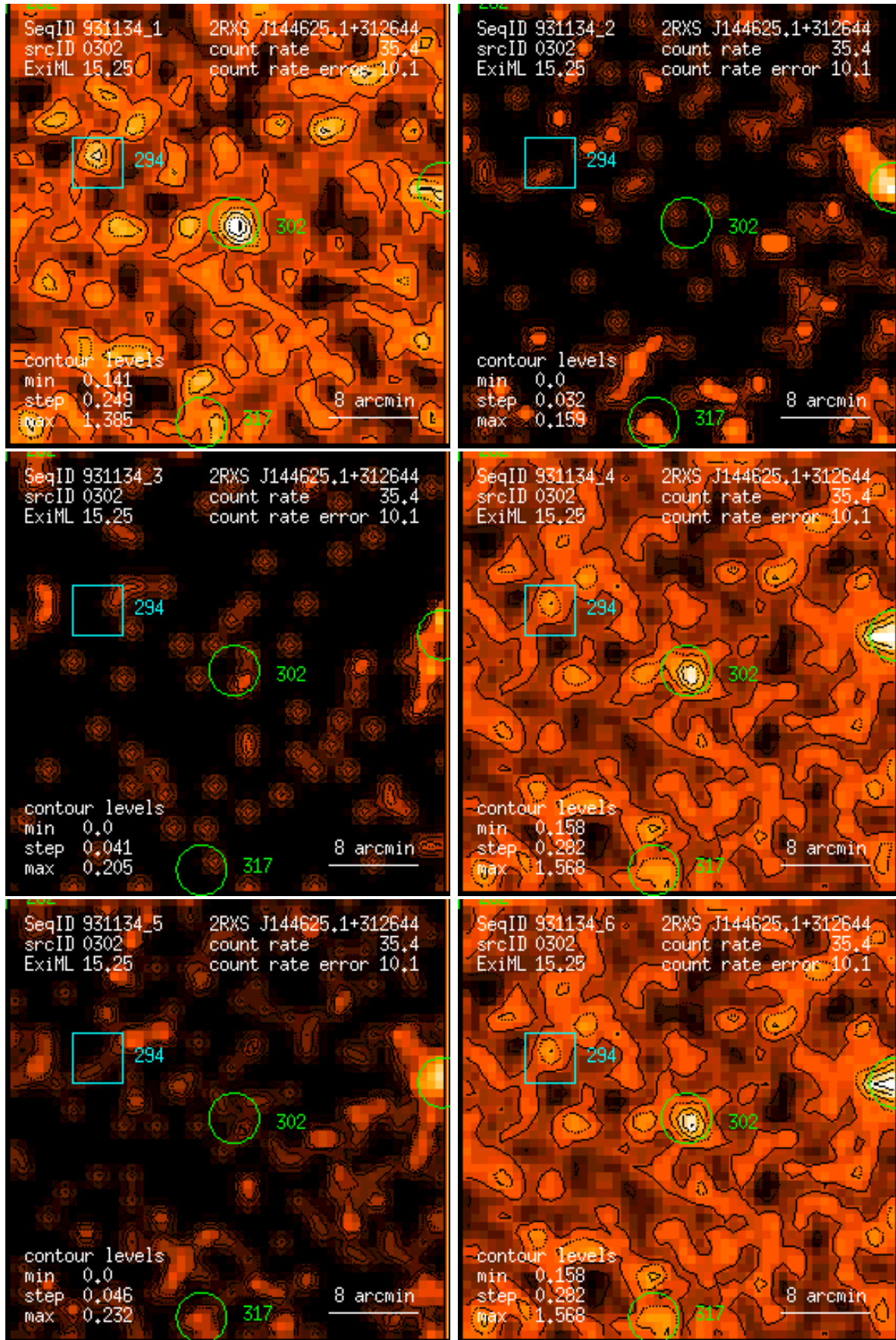
Figure 302: RASS 931134: detection 0302: band rate images, Gaussian filter: (1) PSPC channels 11 – 41, (2) 52 – 90, (3) 91 – 201, (4) 11 – 235, (5) 52 – 201, (6) 11 – 201. Broad band rates in counts/ks. Band rate contour levels in counts/ks/arcmin 2 .
