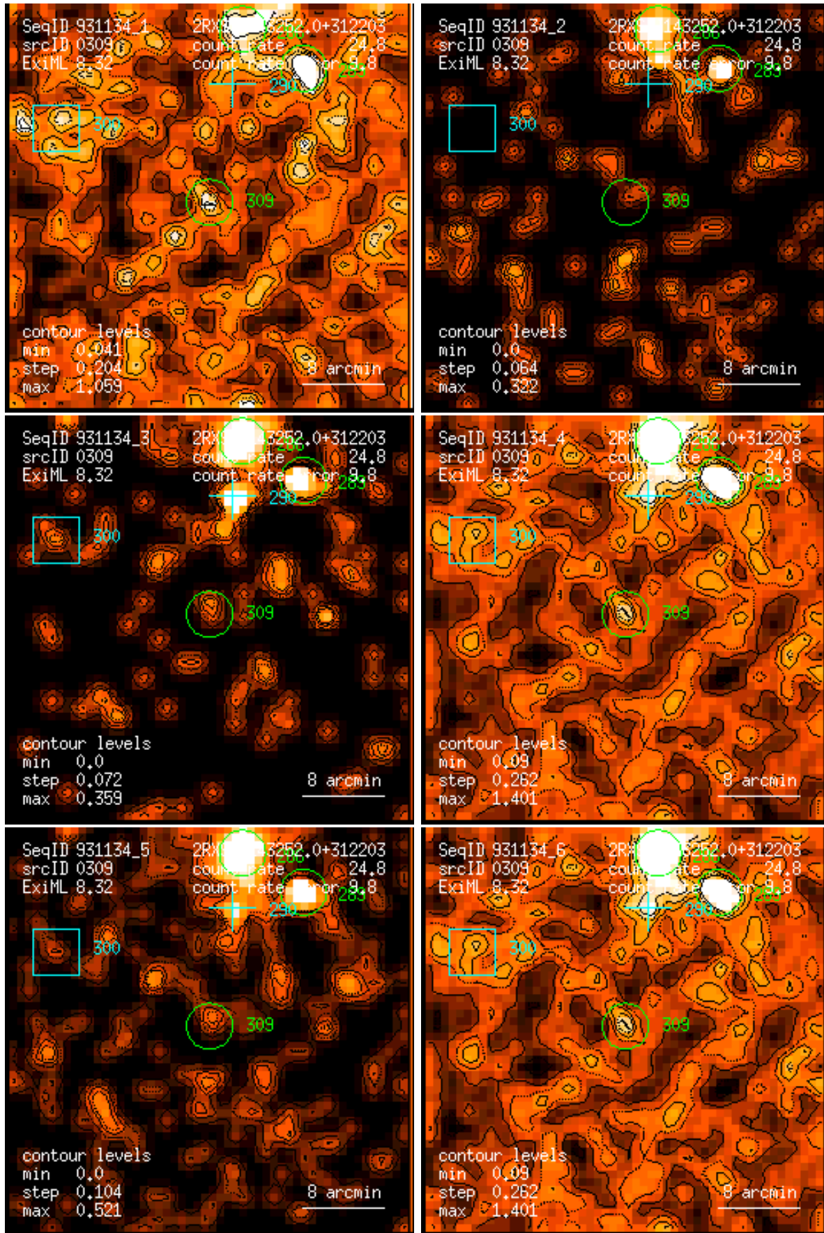
Figure 309: RASS 931134: detection 0309: band rate images, Gaussian filter: (1) PSPC channels 11 – 41, (2) 52 – 90, (3) 91 – 201, (4) 11 – 235, (5) 52 – 201, (6) 11 – 201. Broad band rates in counts/ks. Band rate contour levels in counts/ks/arcmin 2 .
