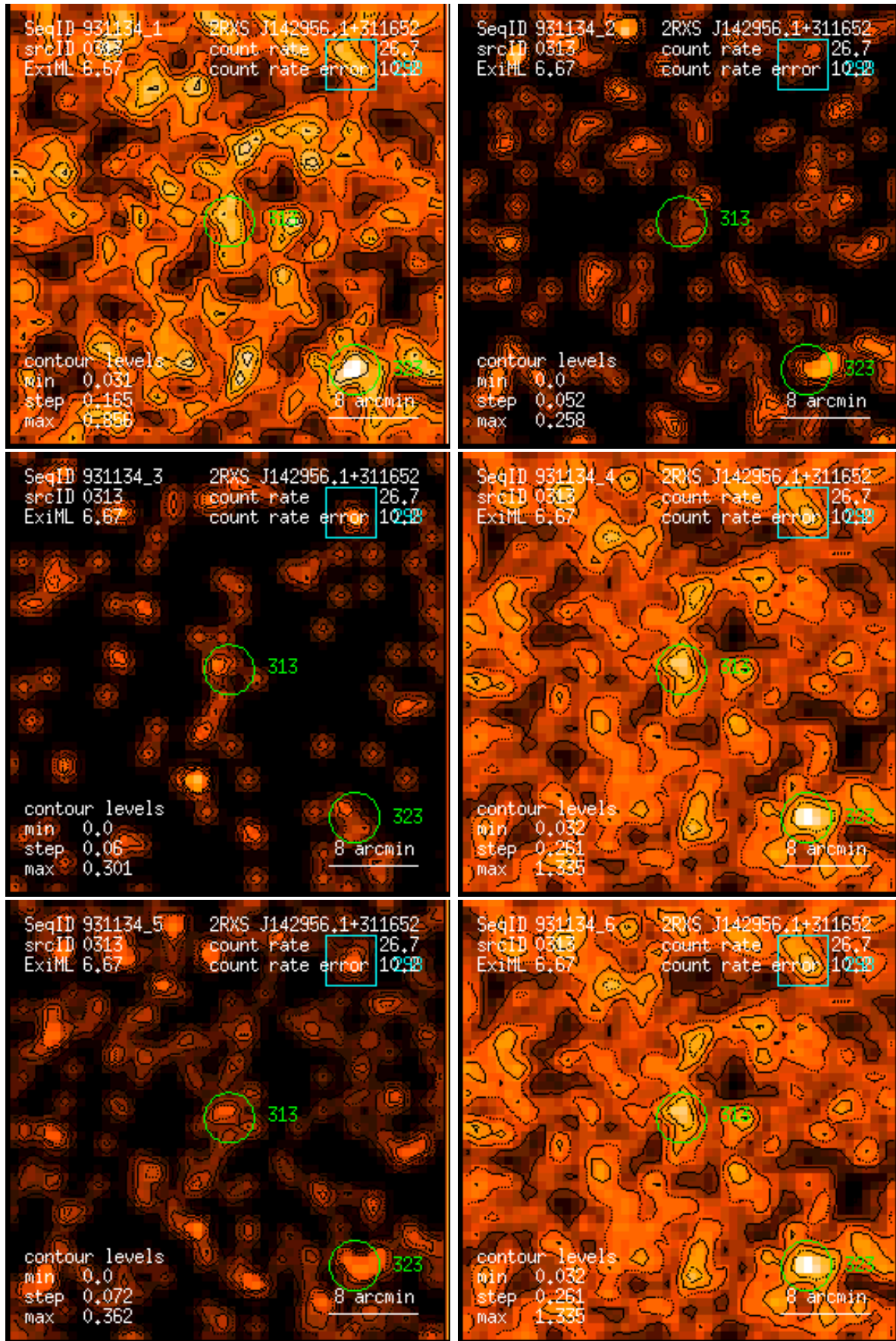
Figure 313: RASS 931134: detection 0313: band rate images, Gaussian filter: (1) PSPC channels 11 – 41, (2) 52 – 90, (3) 91 – 201, (4) 11 – 235, (5) 52 – 201, (6) 11 – 201. Broad band rates in counts/ks. Band rate contour levels in counts/ks/arcmin 2 .
