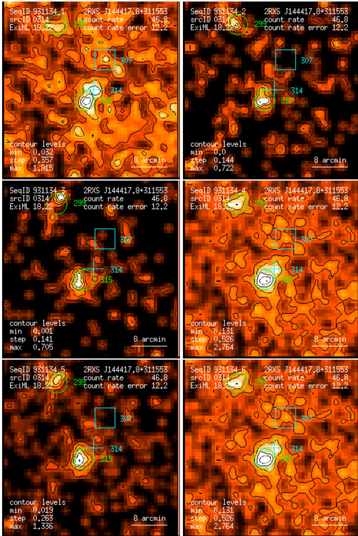
Figure 314: RASS 931134: detection 0314: band rate images, Gaussian filter: (1) PSPC channels 11 – 41, (2) 52 – 90, (3) 91 – 201, (4) 11 – 235, (5) 52 – 201, (6) 11 – 201. Broad band rates in counts/ks. Band rate contour levels in counts/ks/arcmin 2 .
